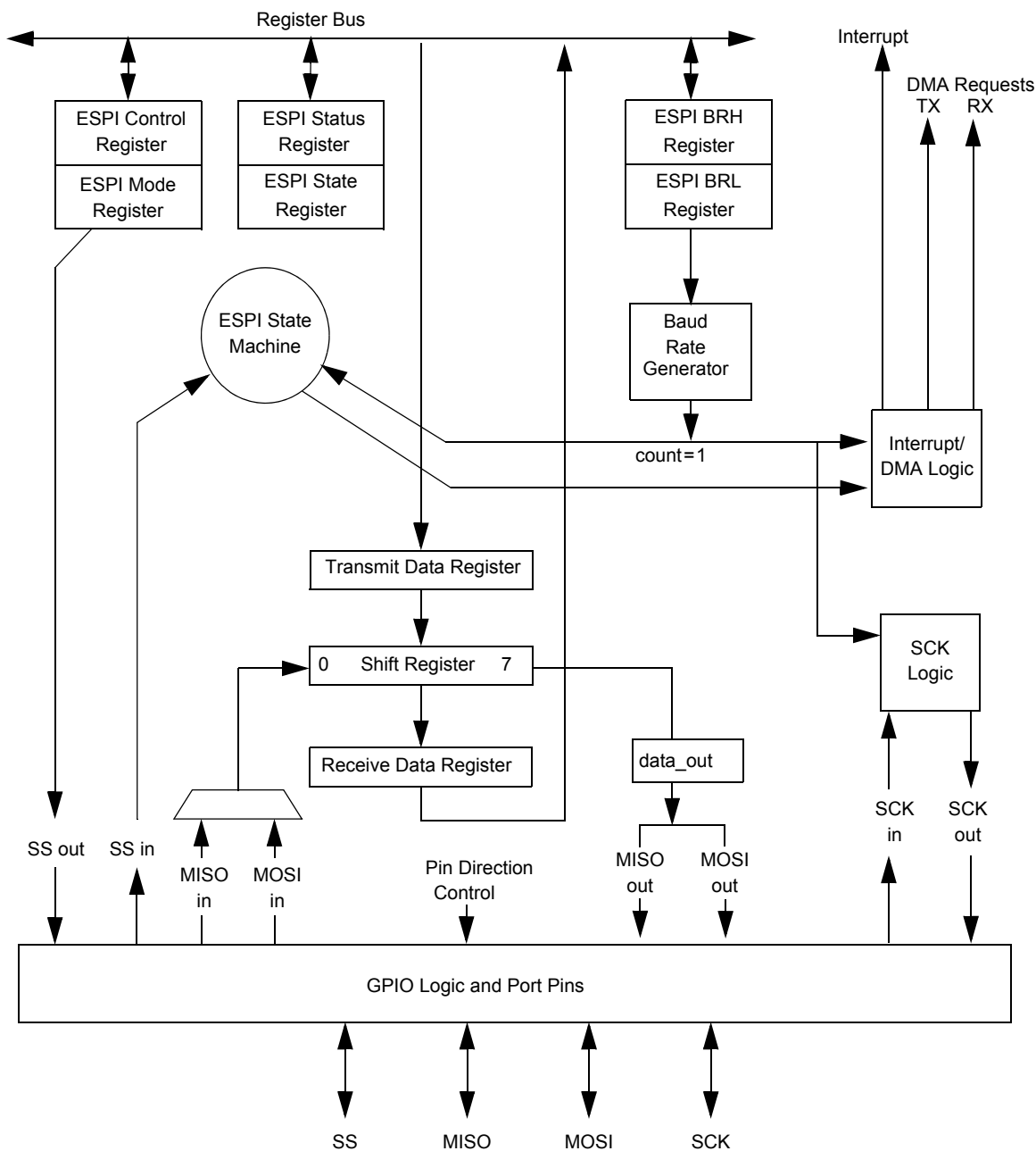
Figure 37. ESPI Block Diagram
