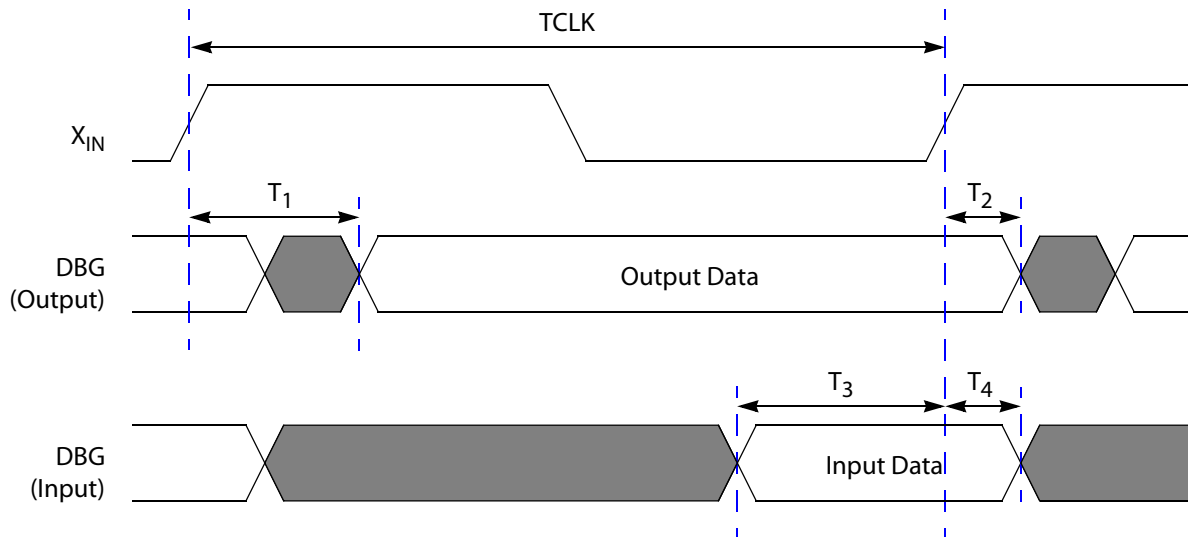
Figure 109. On-Chip Debugger Timing
