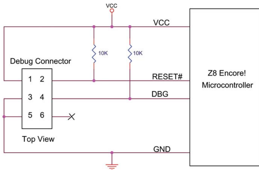
Figure 97. Target OCD Connector Interface
