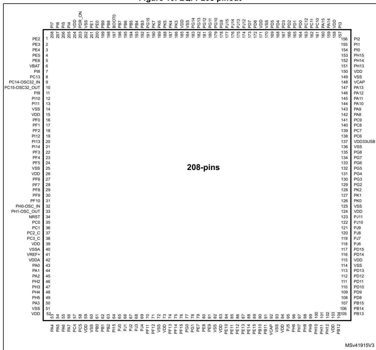
Figure 10. LQFP208 pinout
