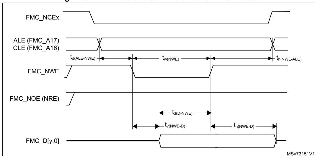
Figure 82. NAND controller waveforms for write access
