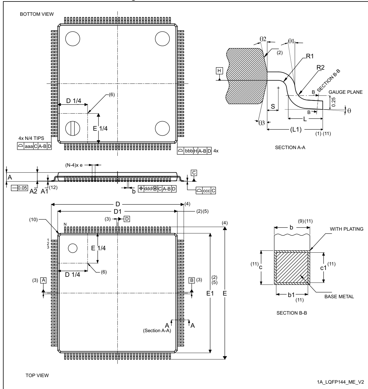
Figure 119. LQFP144 - Outline (15)
