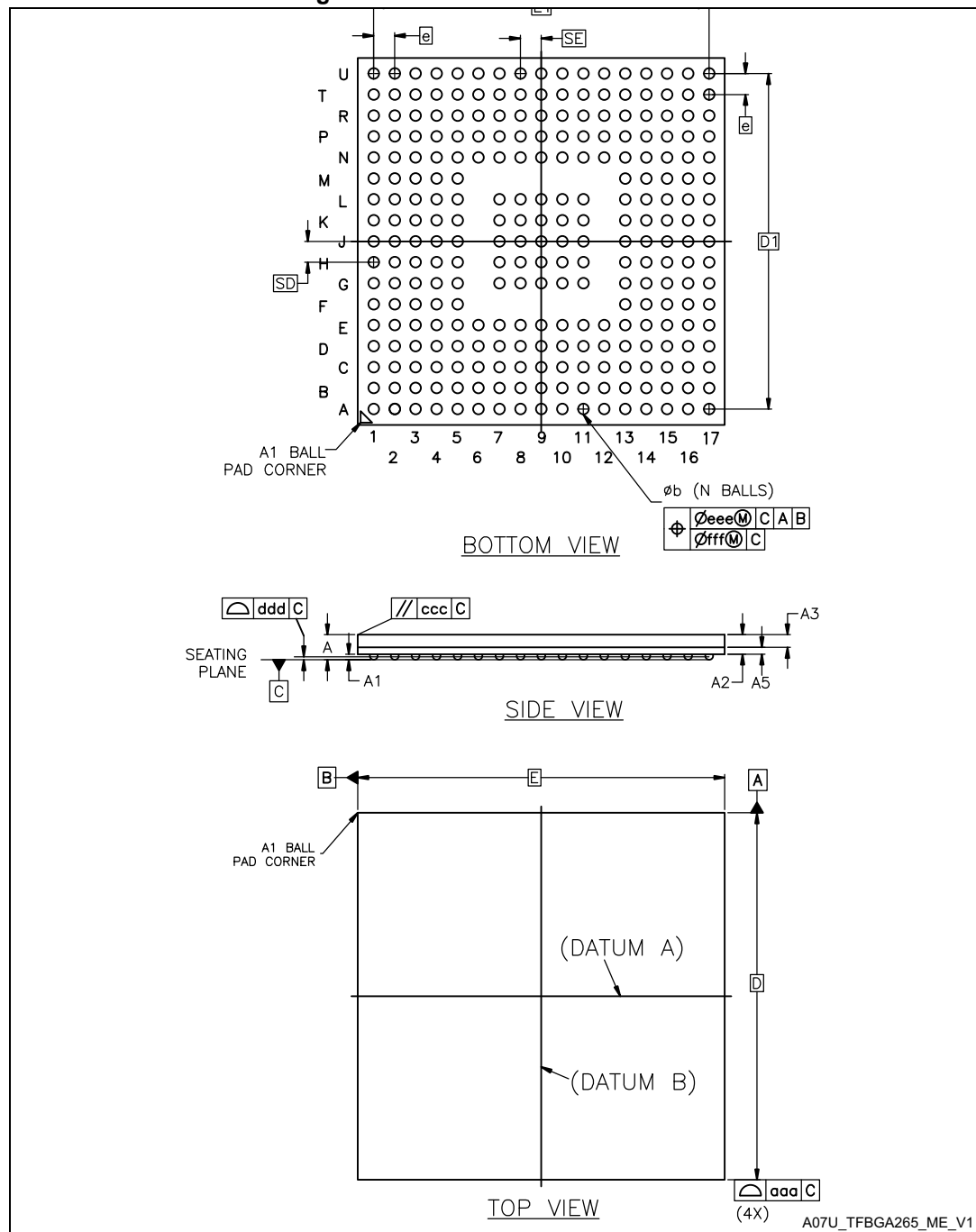
Figure 129. TFBGA240+25 - Outline
