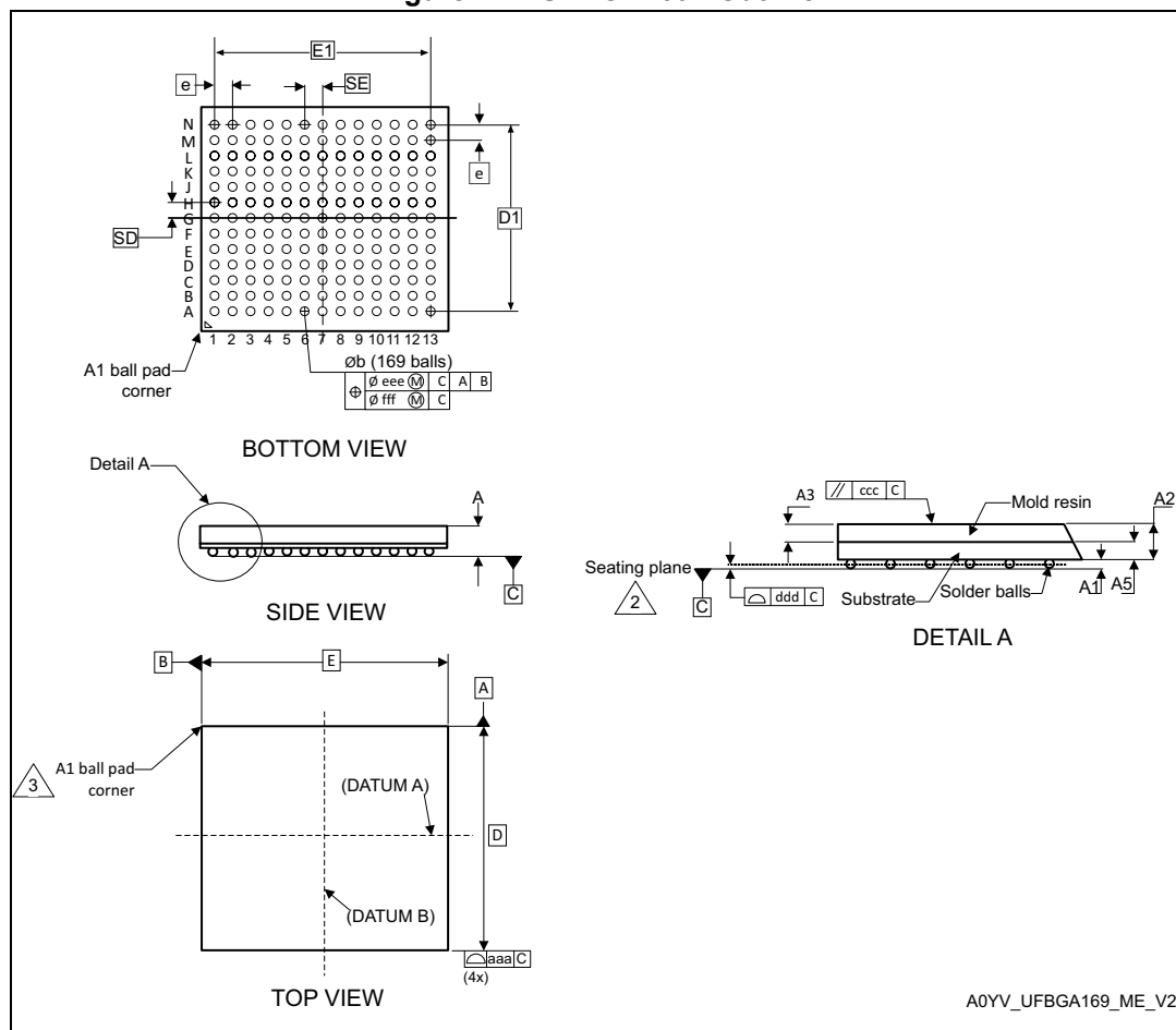
Figure 121. UFBGA169 - Outline
