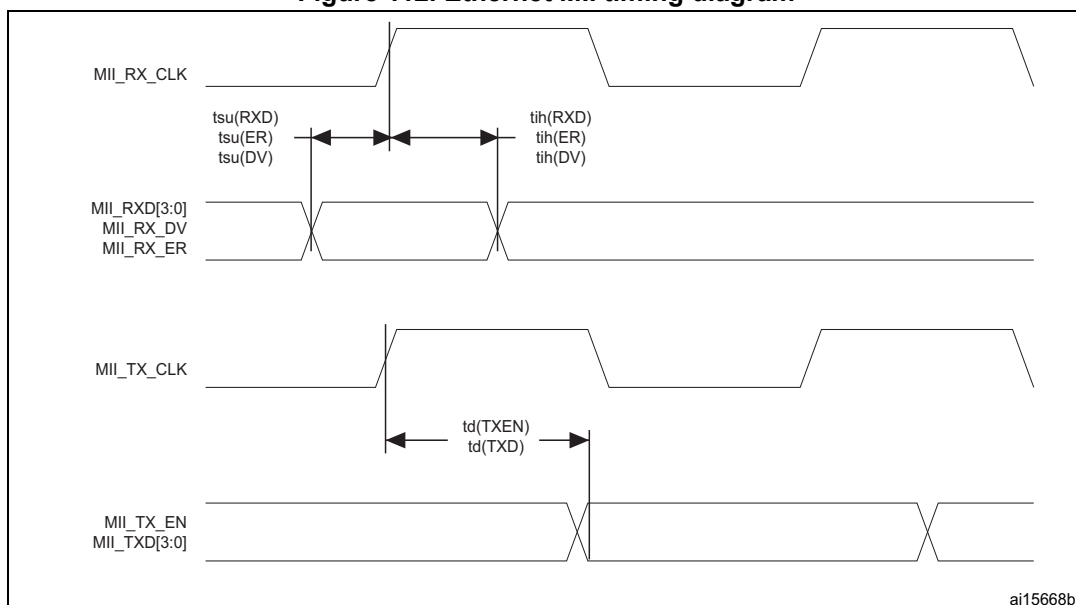
Figure 112. Ethernet MII timing diagram
