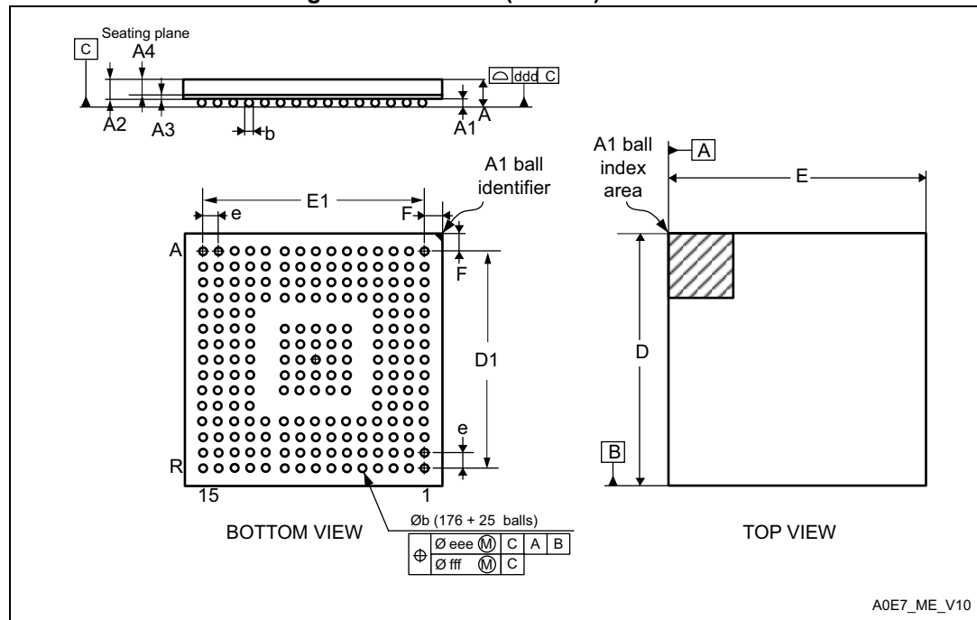
Figure 127. UFBGA(176+25) - Outline
