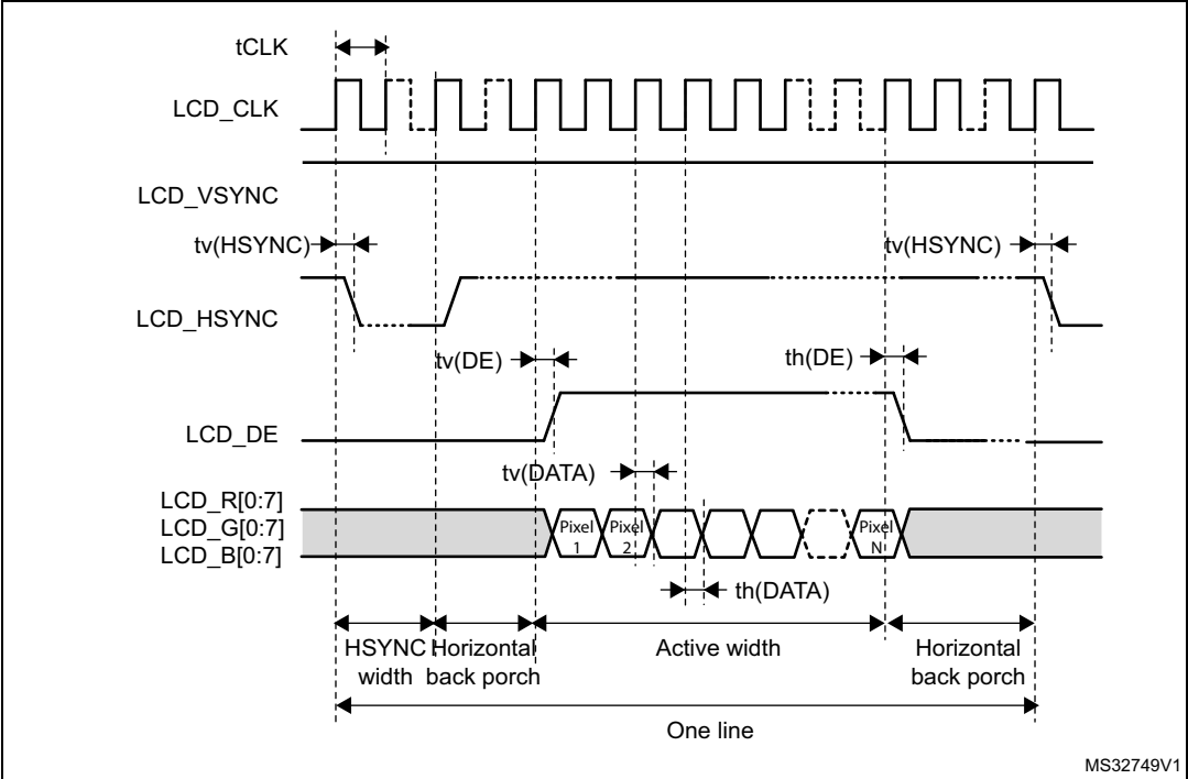
Figure 94. LCD-TFT horizontal timing diagram
