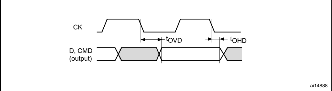
Figure 55. SD default mode
