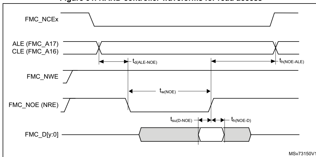
Figure 31. NAND controller waveforms for read access
