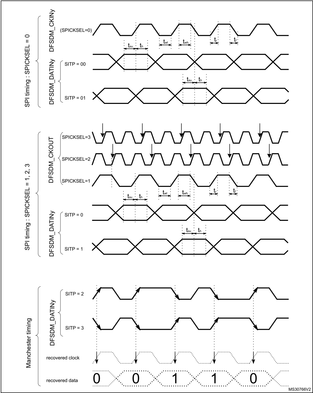
Figure 92. Channel transceiver timing diagrams
