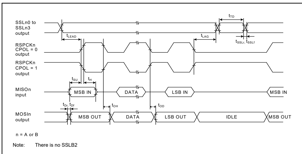
Figure 48.51 SPI timing (master, CPHA = 0) (bit rate: PCLKA division ratio is set to any value other than 1/2)
