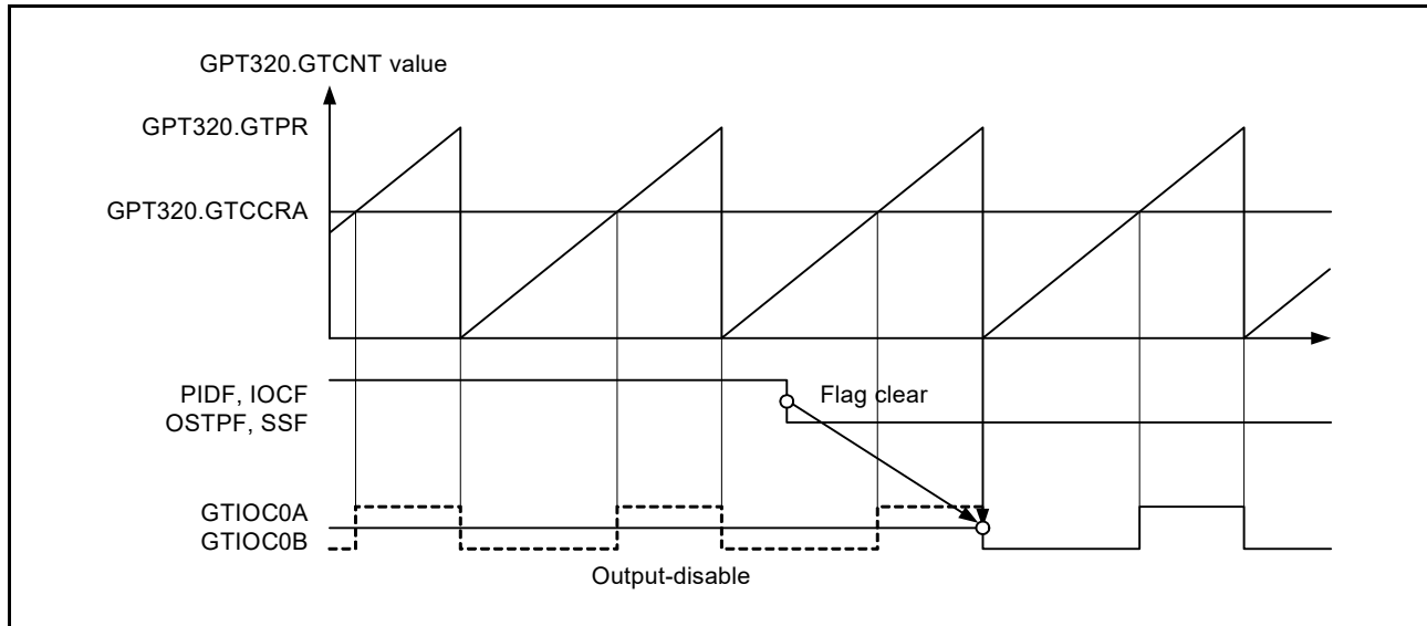
Figure 22.3 Output-disable release timing for GPT pin outputs
