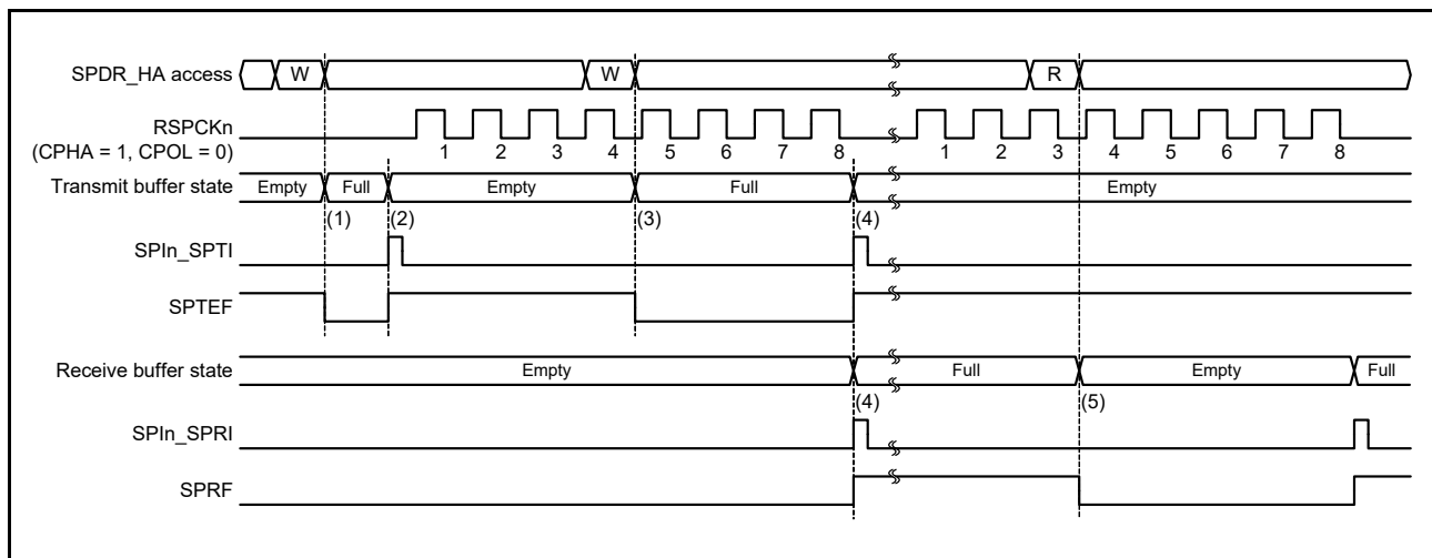
Figure 32.31 Operation example of SPIn_SPTI and SPIn_SPRI interrupts when CPHA = 1 and CPOL = 0
