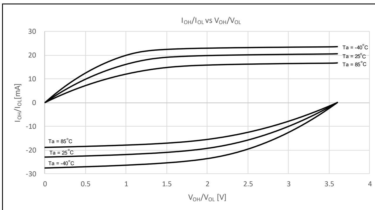
Figure 48.5 V_{OH}/V_{OL} and I_{OH}/I_{OL} temperature characteristics at V_{CC} = 3.6 V when low drive output is selected (reference data)
