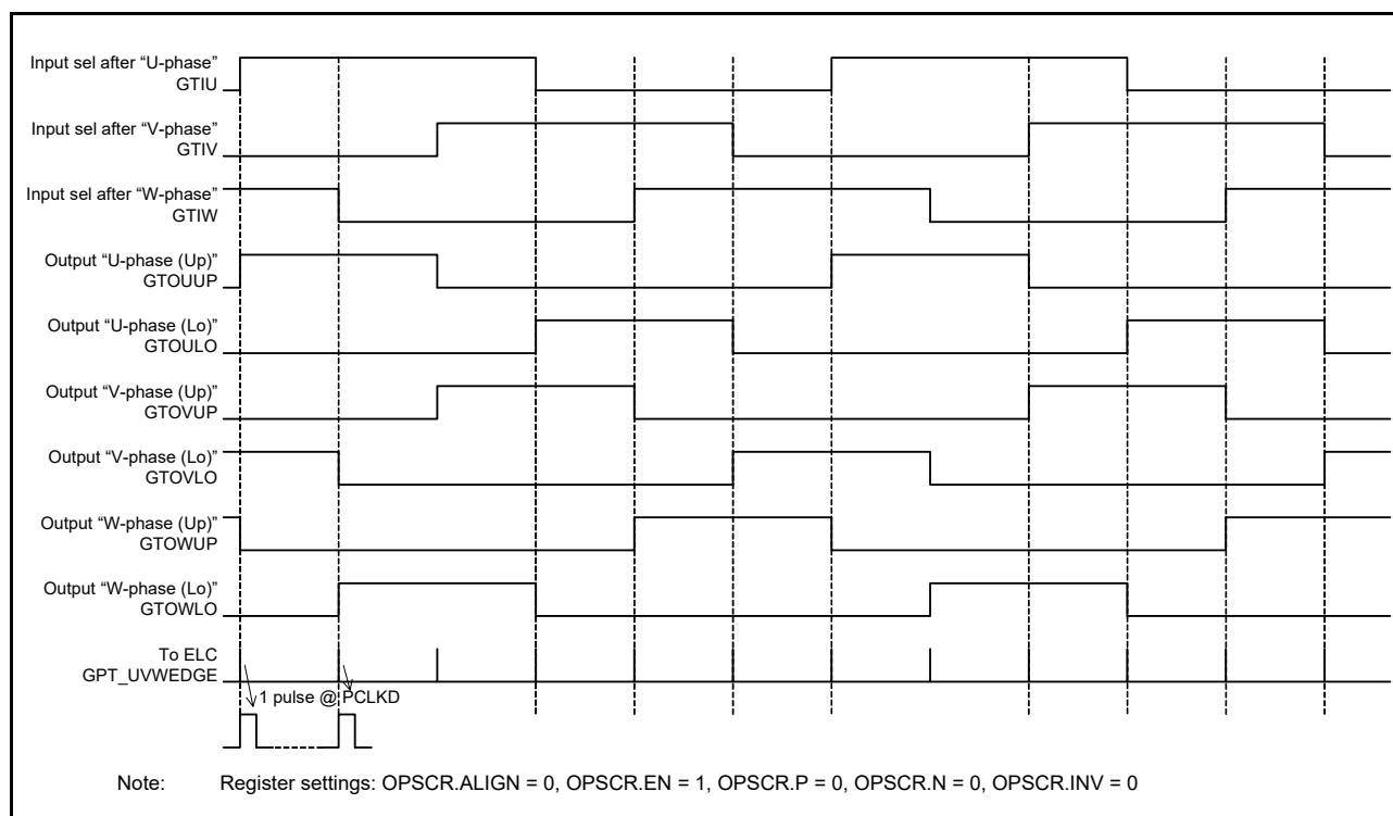
Figure 23.78 Example of 6-phase level output operation
