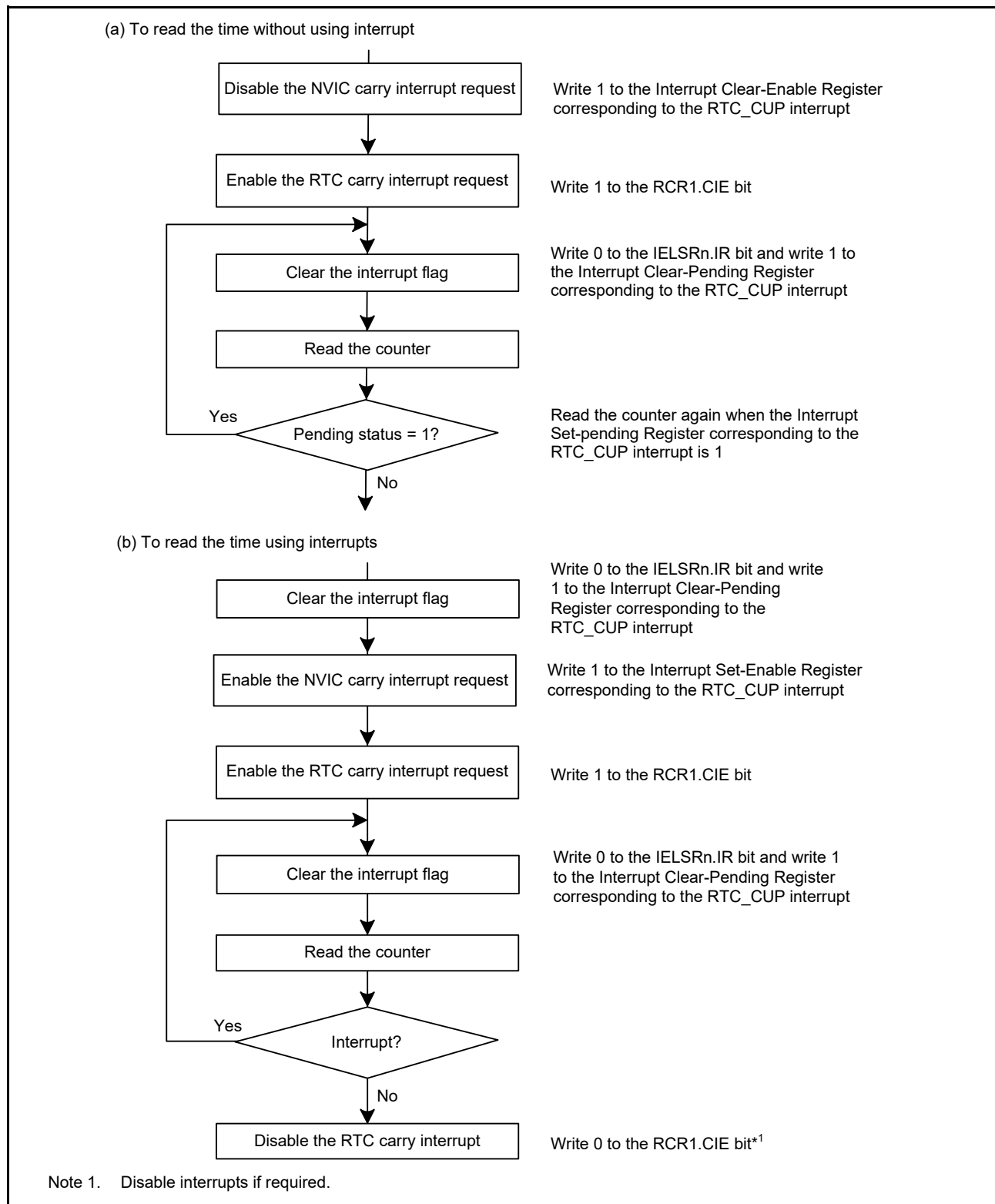
Figure 25.6 Reading time
