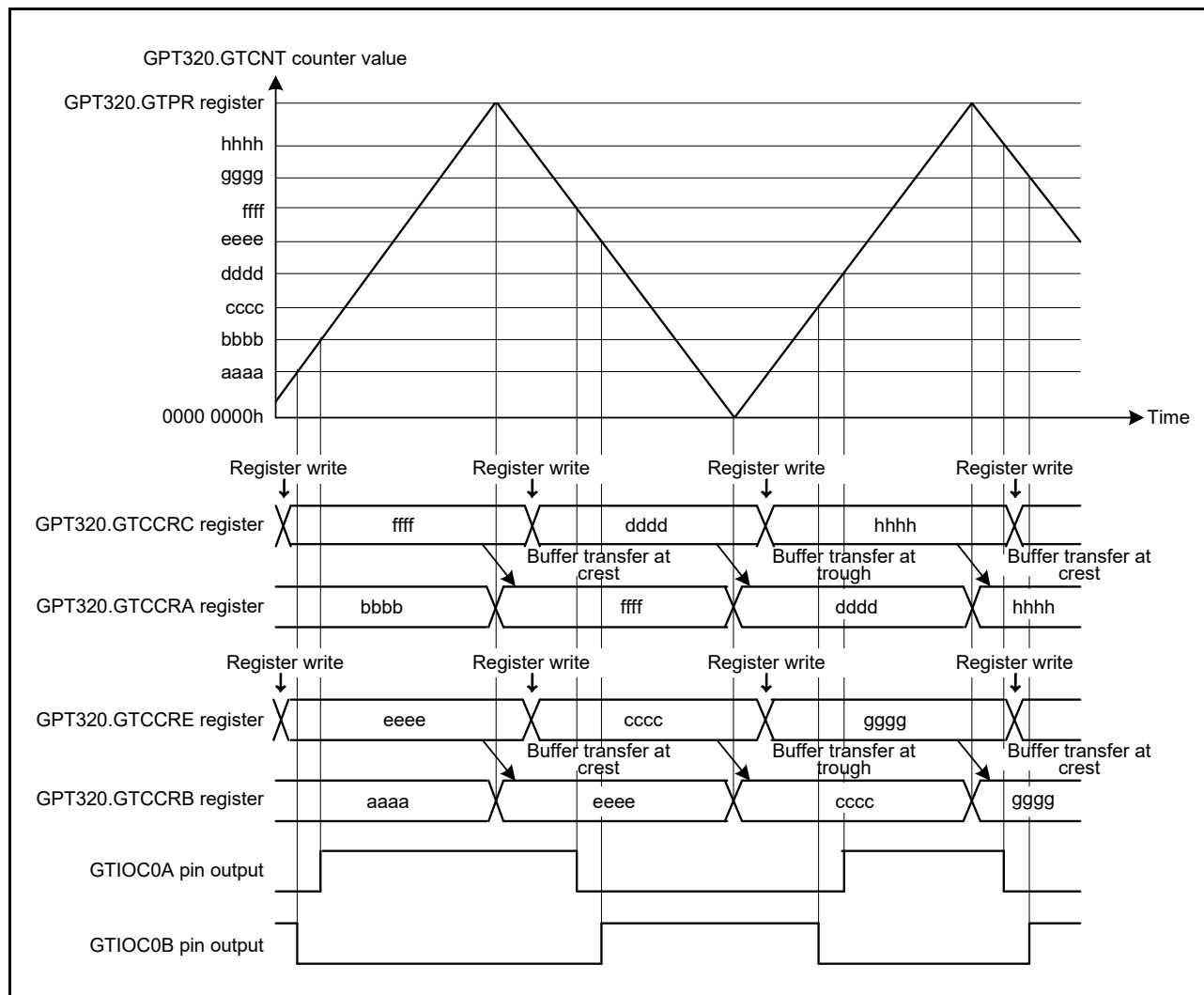
Figure 23.35 Example of triangle-wave PWM mode 2 operation with buffer operation, low output from the GTIOCA pin and high output from the GTIOCB pin at count start, output toggled at GTCCRA/ GTCCRB compare match, and output retained at cycle end
