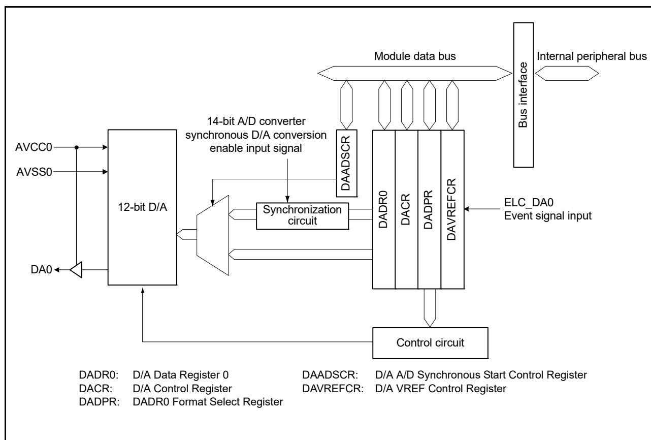
Figure 35.1 DAC12 block diagram
