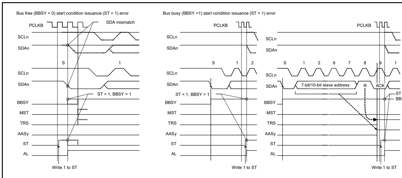
Figure 30.42 Arbitration-loss when start condition is issued (MALE = 1)
