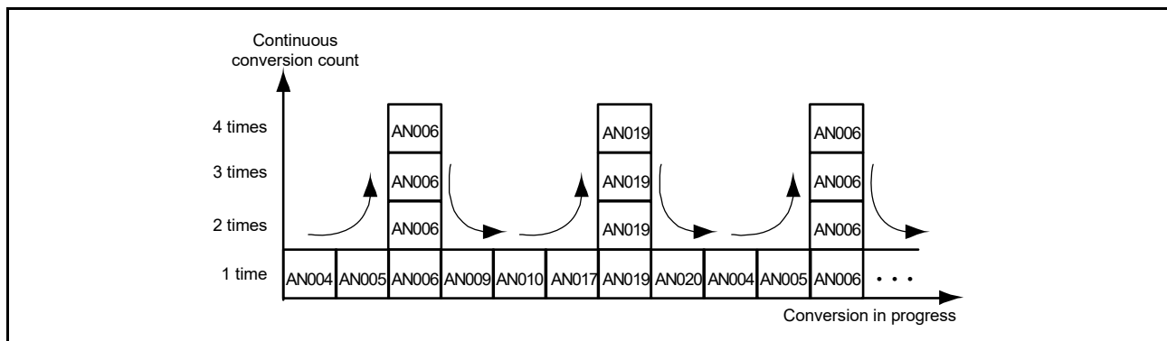
Figure 34.2 Scan conversion sequence with ADADC.ADC[2:0] = 011b, ADADS0.ADS06 = 1, and ADADS1.ADS19 = 1
