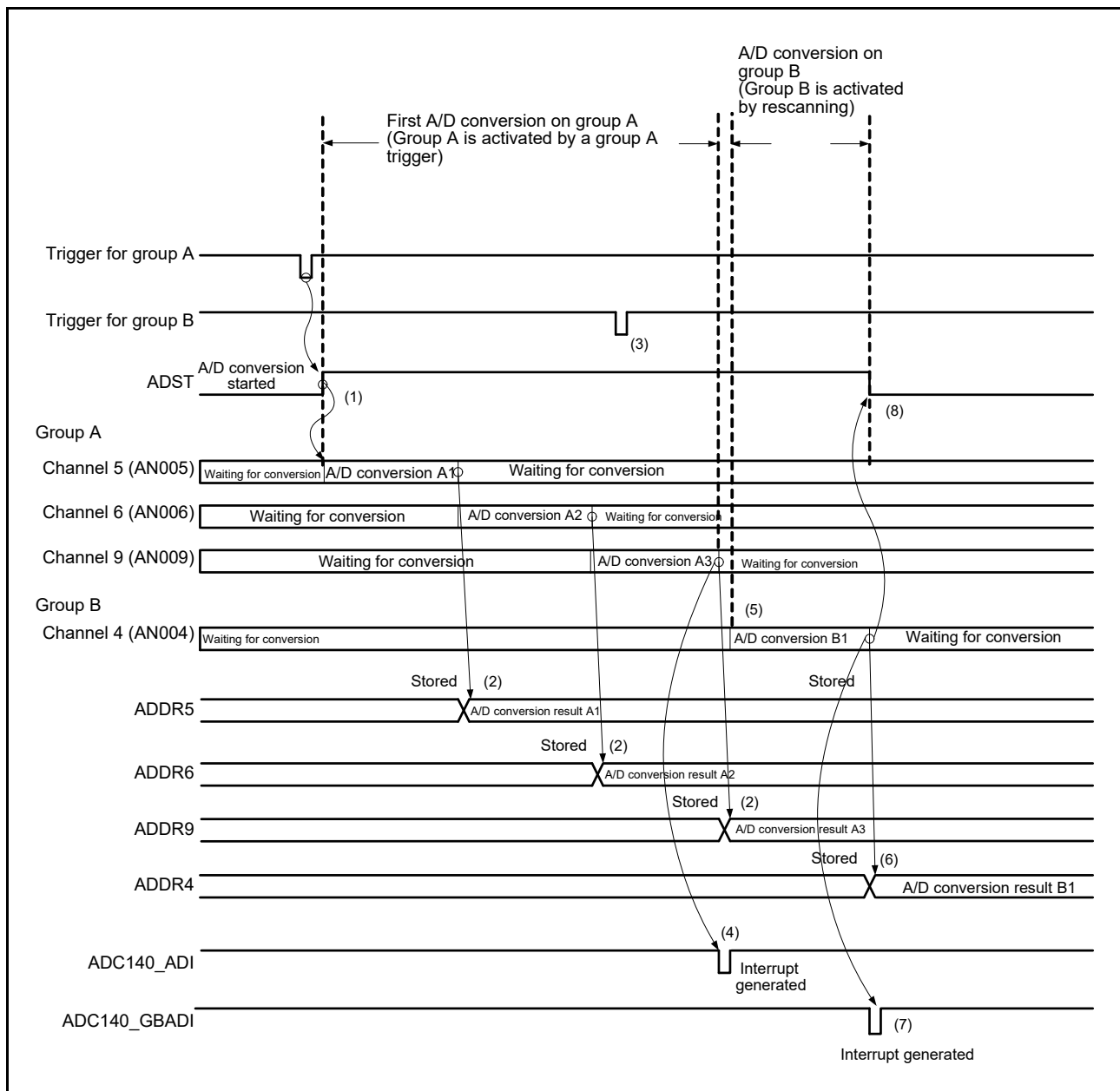
Figure 34.18 Example operation with group A priority control (3), when ADGSPCR.GBRSCN = 1 and ADGSPCR.GBRP = 0
