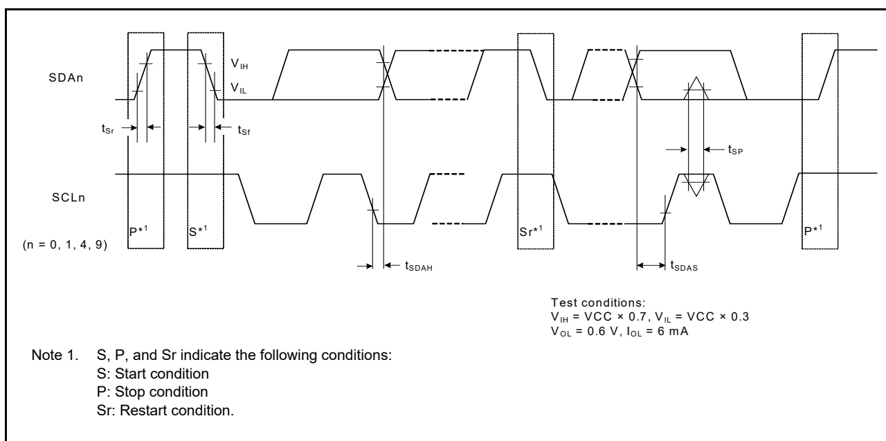
Figure 48.49 SCI simple IIC mode timing
