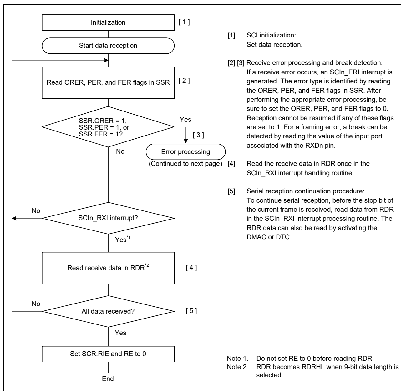
Figure 29.17 Example flow of serial reception in asynchronous mode with non-FIFO selected (1)
