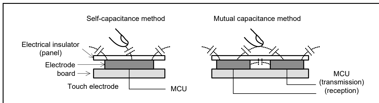
Figure 40.2 Self-capacitance and mutual-capacitance methods
