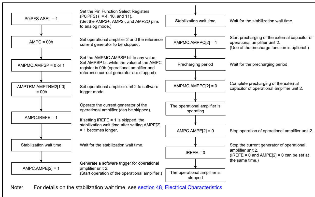
Figure 37.7 Procedure to start and stop OPAMP in software trigger mode
