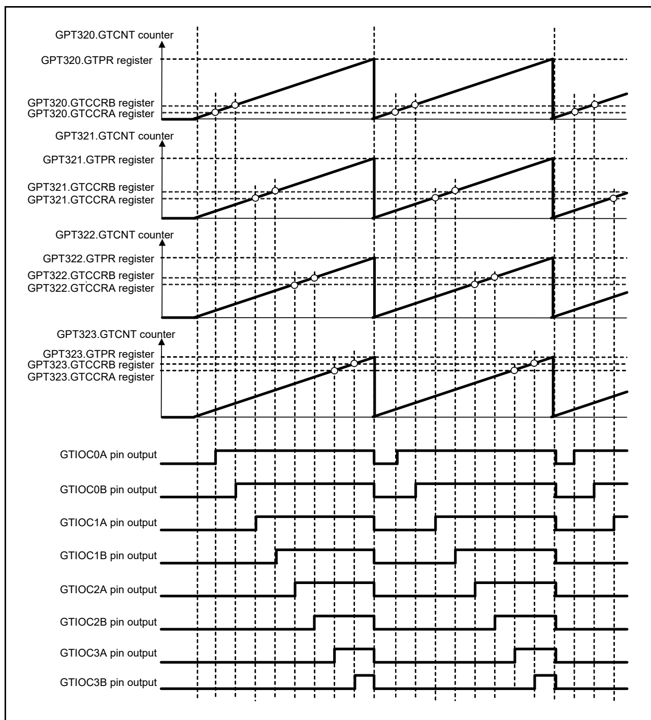
Figure 23.61 Example of synchronized PWM output
