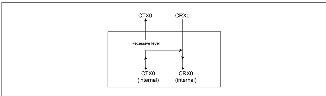
Figure 31.6 Connection when listen-only mode is selected
