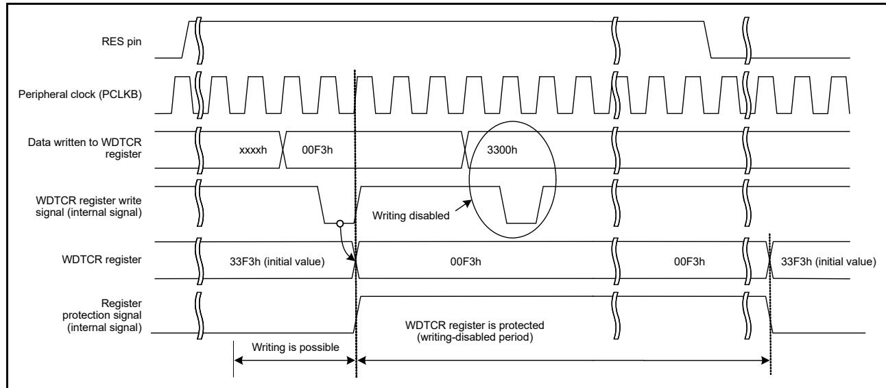
Figure 26.5 Control waveforms produced in response to writes to the WDTCSR register
