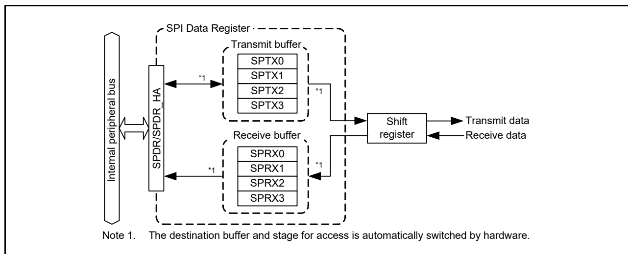
Figure 32.2 Configuration of SPDR/SPDR_HA (SPI0)
