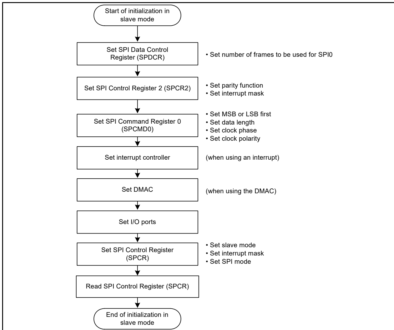
Figure 32.58 Example of initialization flow in slave mode for clock synchronous operation
