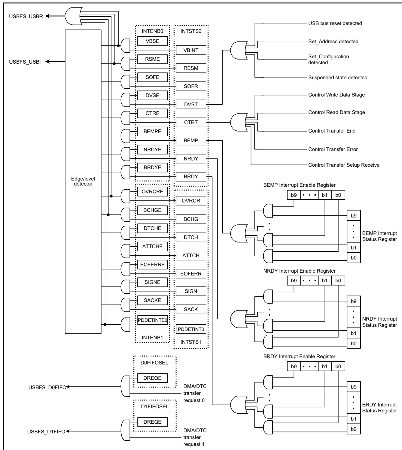
Figure 28.7 USBFS interrupt-related circuits
