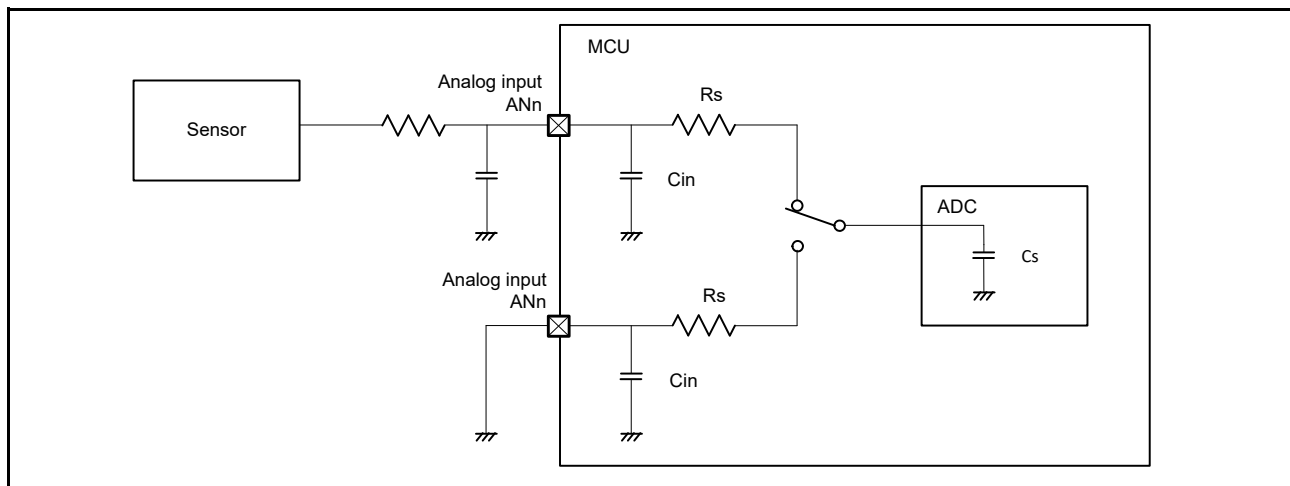
Figure 48.64 Equivalent circuit for analog input
