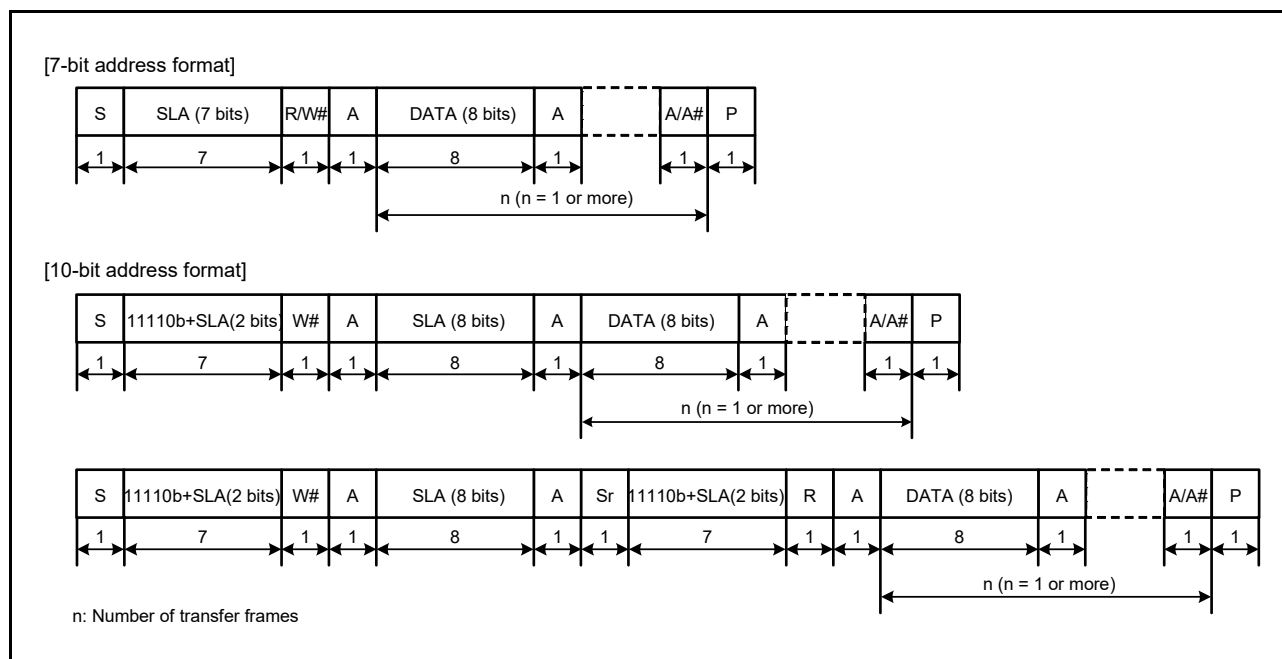
Figure 30.3 I 2 C bus format
