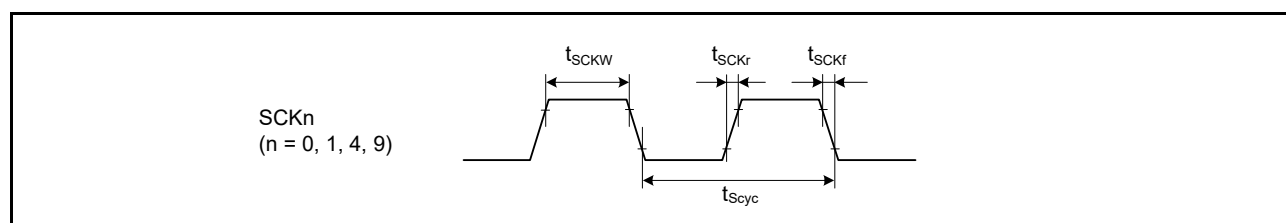
Figure 48.42 SCK clock input timing
