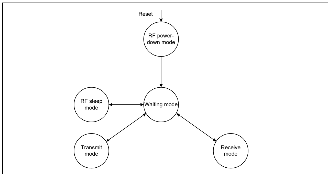
Figure 46.2 State Transition Diagram of the BLE
