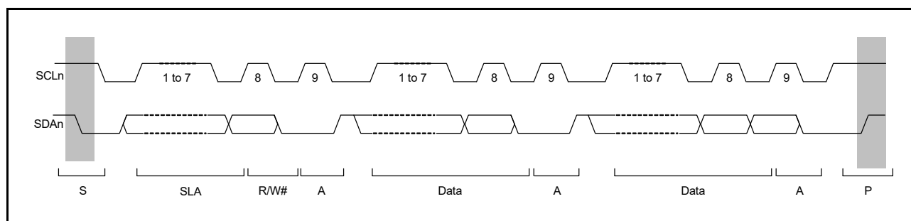
Figure 30.4 I 2 C bus timing (SLA = 7 bits)
