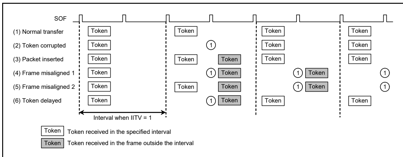
Figure 28.19 Example interval error occurrence when IITV = 1
