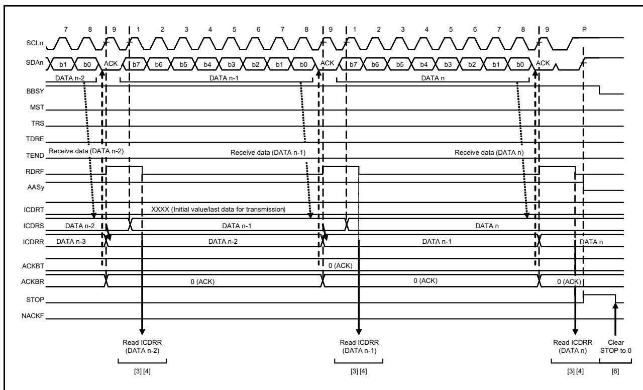
Figure 30.20 Slave receive operation timing (2) when RDRFS = 0
