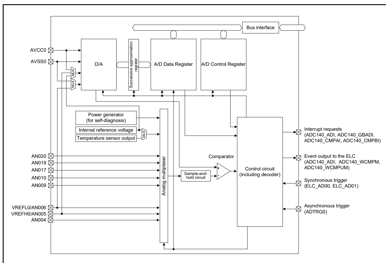
Figure 34.1 ADC14 block diagram
