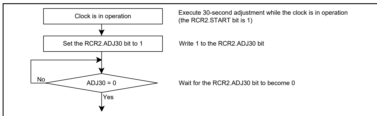
Figure 25.5 30-second adjustment
