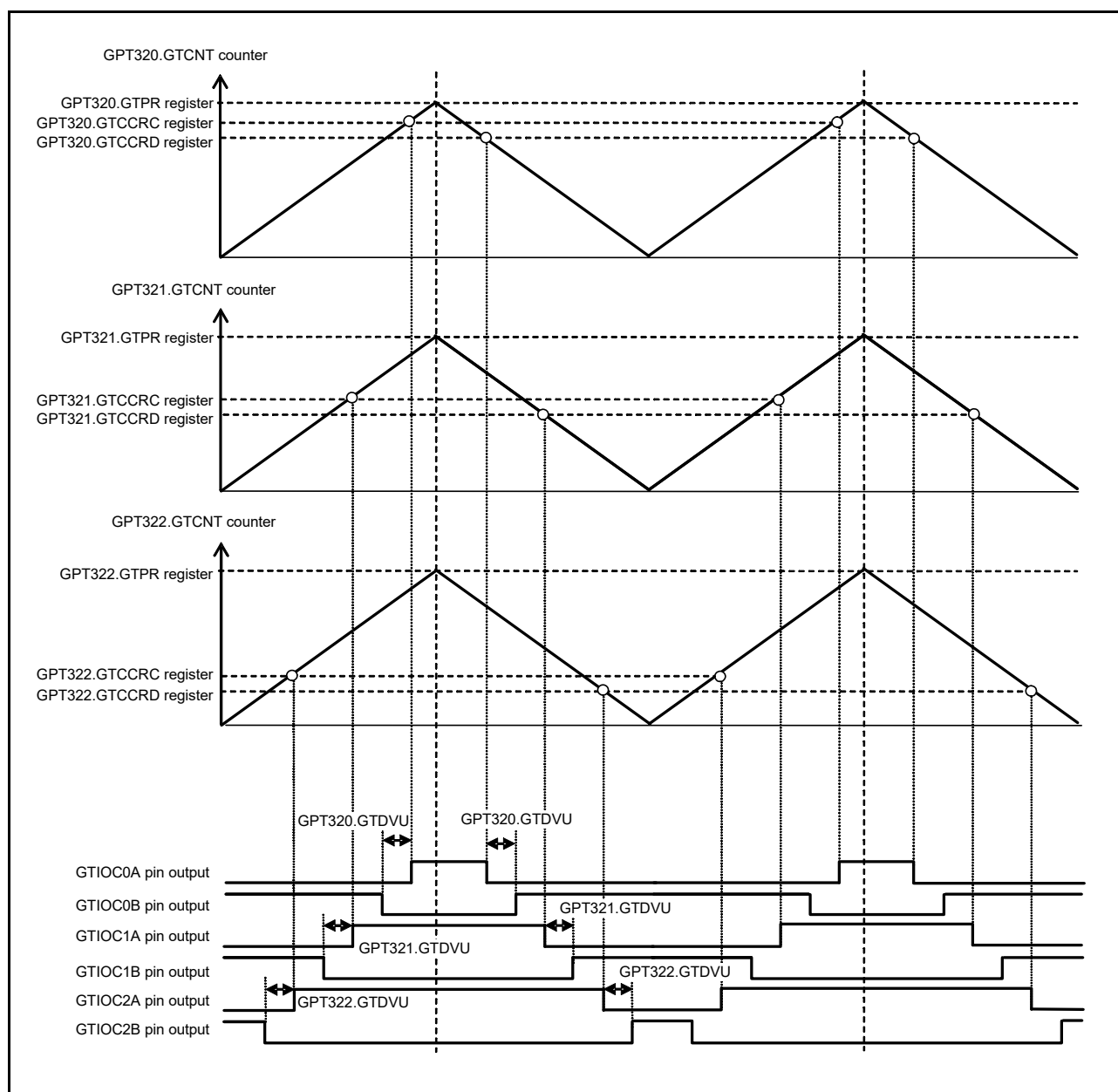
Figure 23.66 Example of 3-phase asymmetric triangle-wave complementary PWM output with automatic dead time setting
