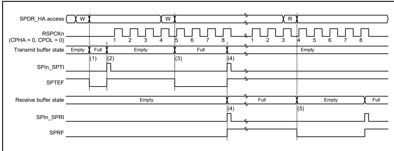
Figure 32.30 Operation example of SPIn_SPTI and SPIn_SPRI interrupts when CPHA = 0 and CPOL = 0
