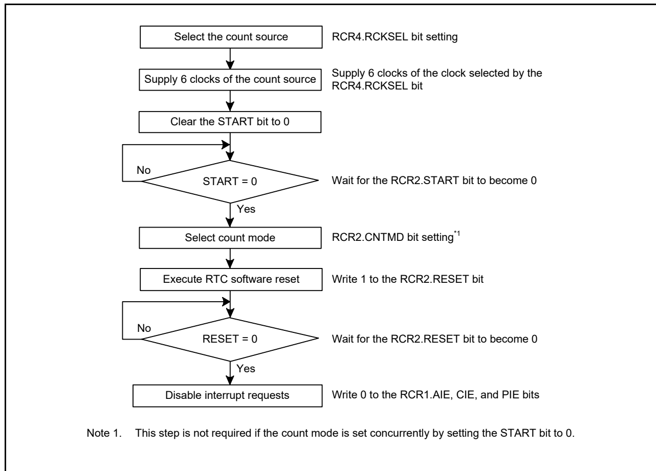
Figure 25.14 Initialization procedure
