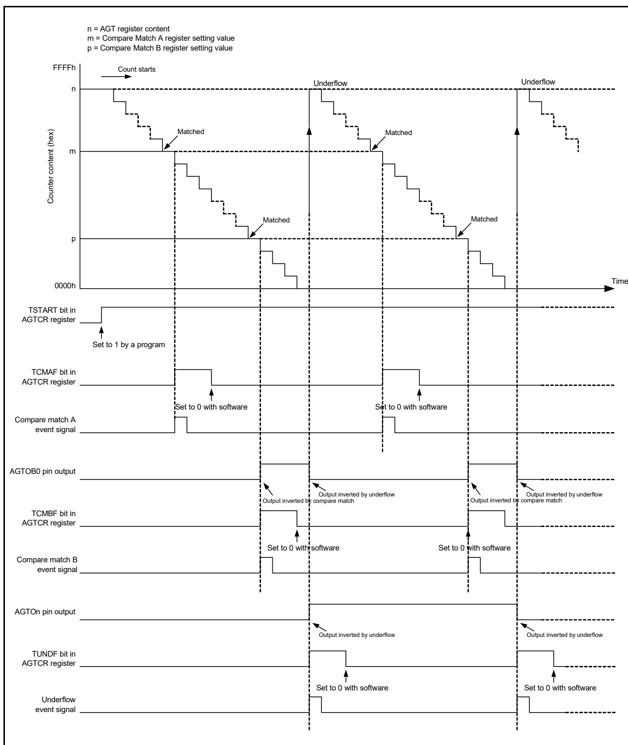
Figure 24.11 Operation example in compare match mode (TOPOLB = 0)
