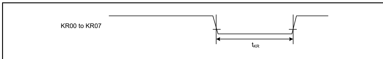
Figure 48.41 Key interrupt input timing
