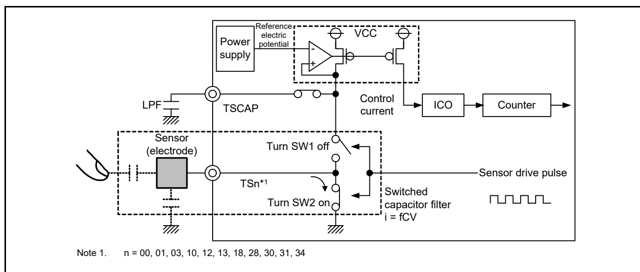
Figure 40.6 Discharging operation
