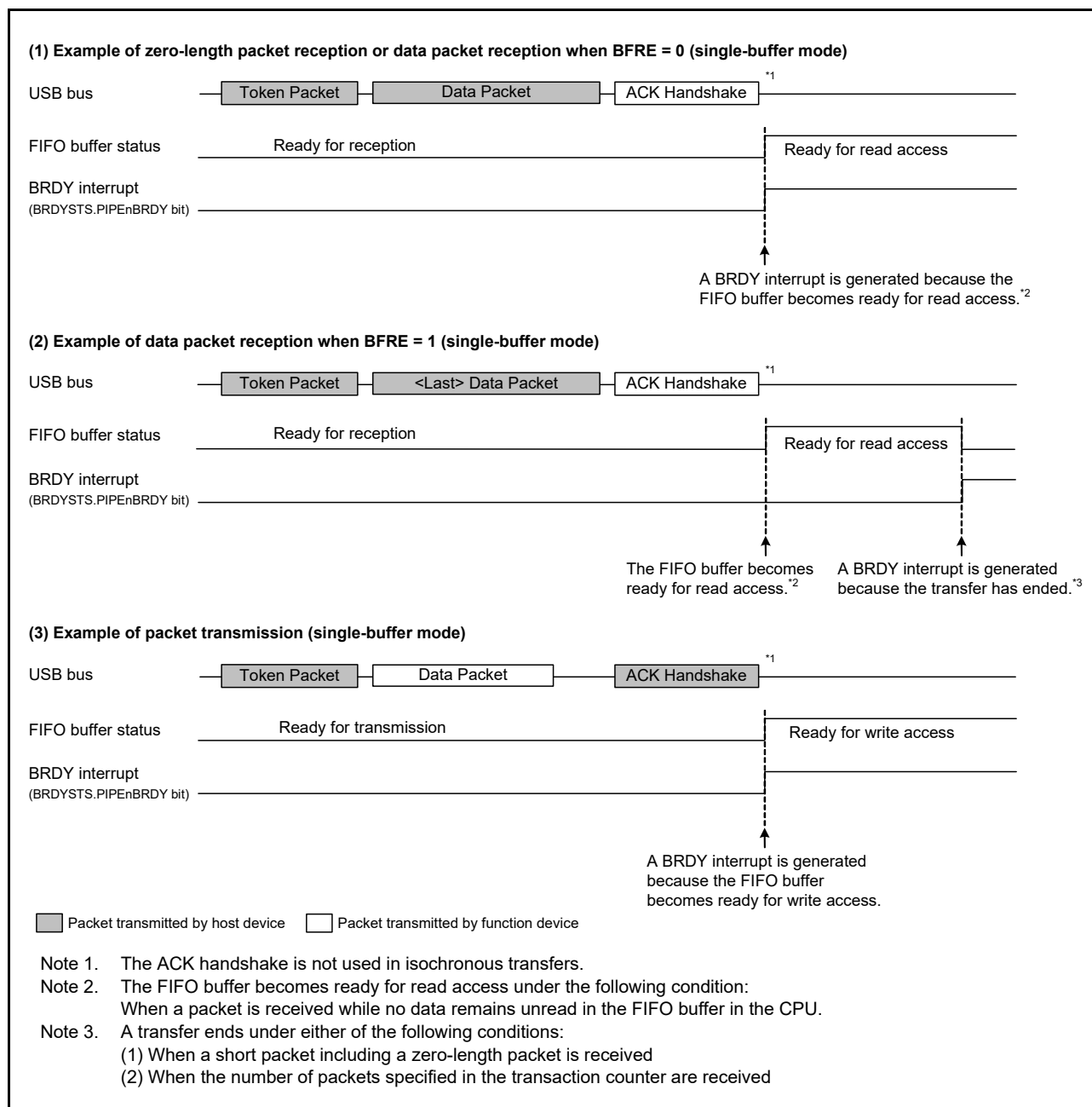
Figure 28.8 Timing of BRDY interrupt generation
