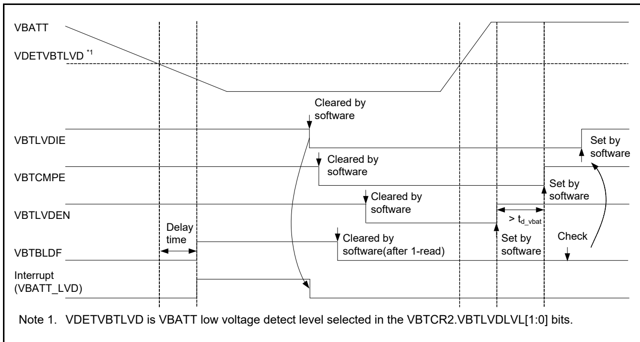
Figure 12.4 Basic operation of VBATT low voltage detection interrupt
