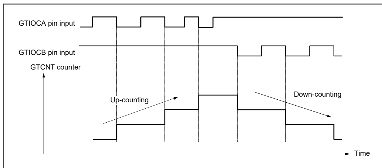
Figure 23.71 Example of phase counting mode 3 (A)
