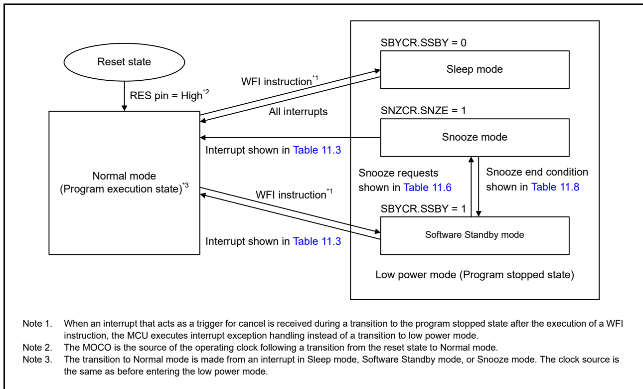
Figure 11.1 Mode transitions
