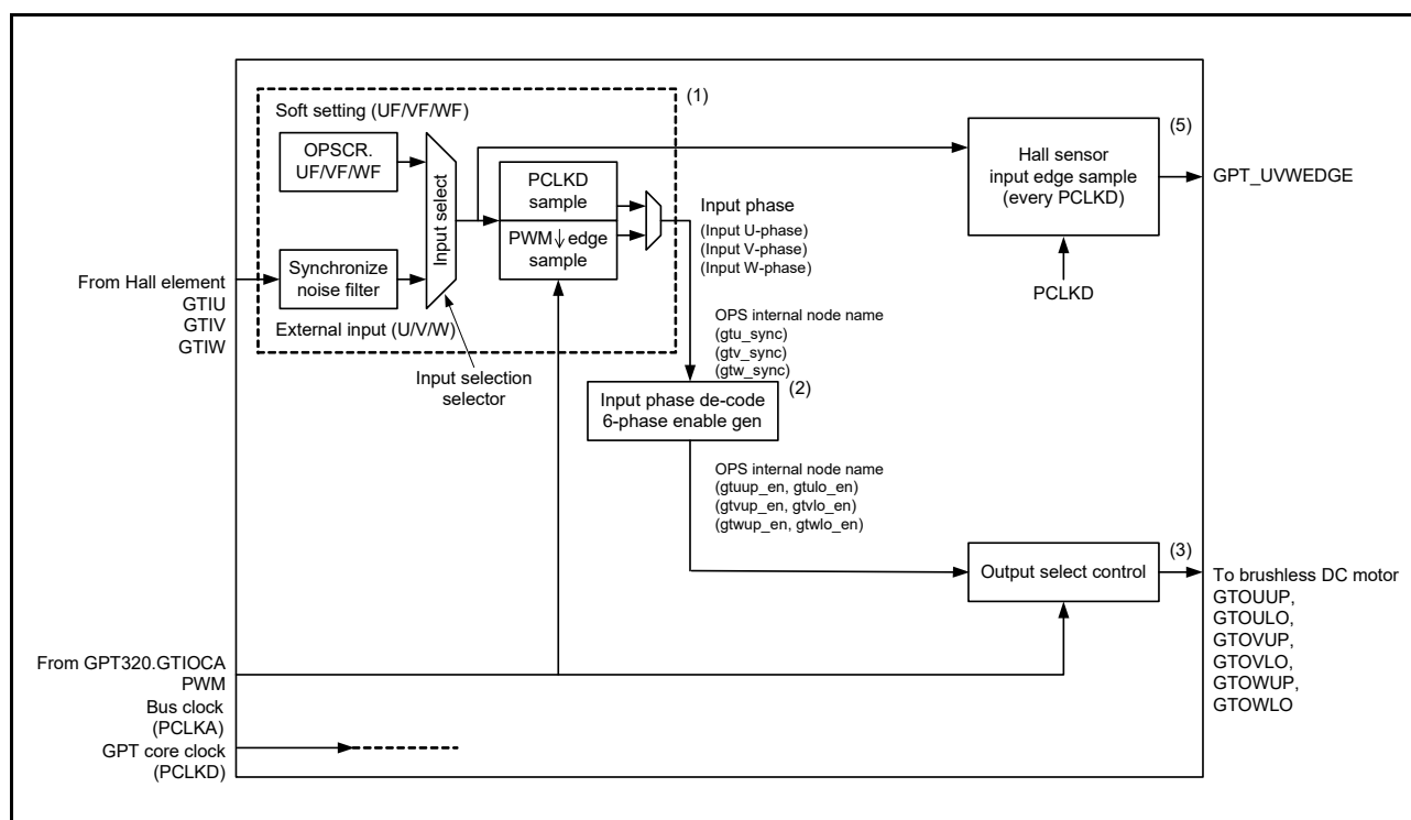
Figure 23.77 Conceptual diagram of GPT_OPS control flow
