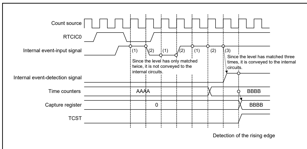
Figure 25.10 Timing of a time capture operation with the filter on
