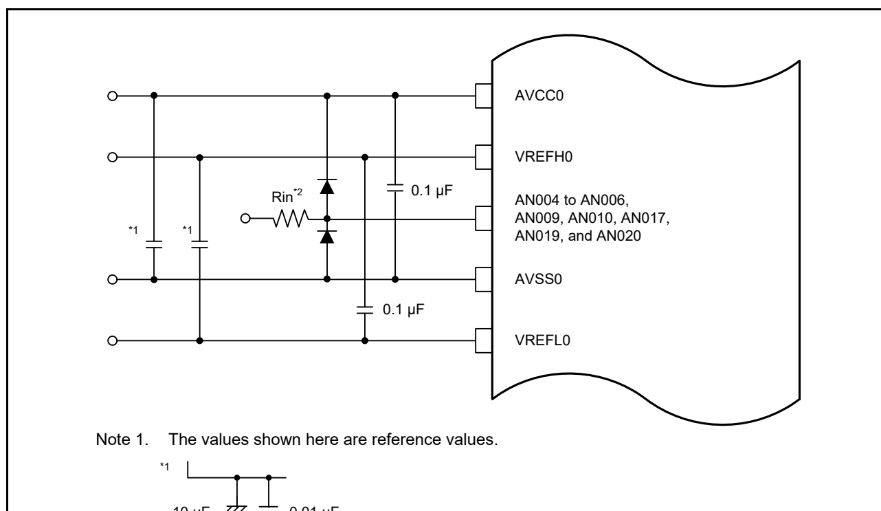
Figure 34.32 Example protection circuit for analog inputs
