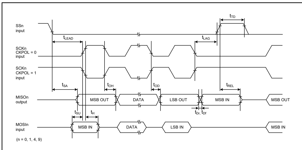
Figure 48.47 SCI simple SPI mode timing (slave, CKPH = 1)
