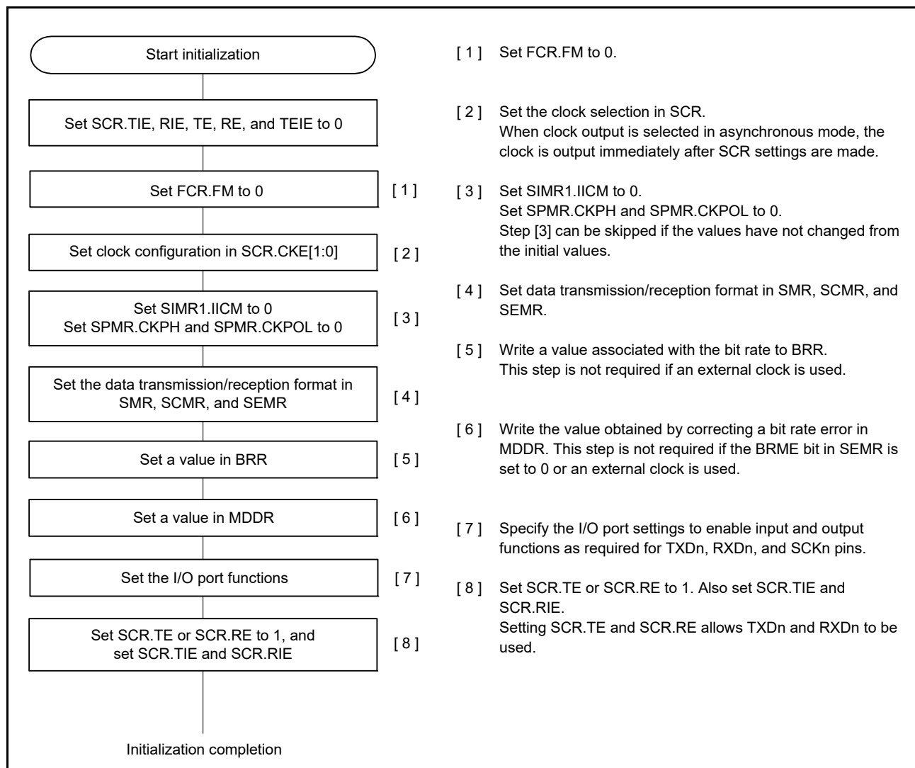
Figure 29.7 Example SCI initialization flow in asynchronous mode with non-FIFO selected
