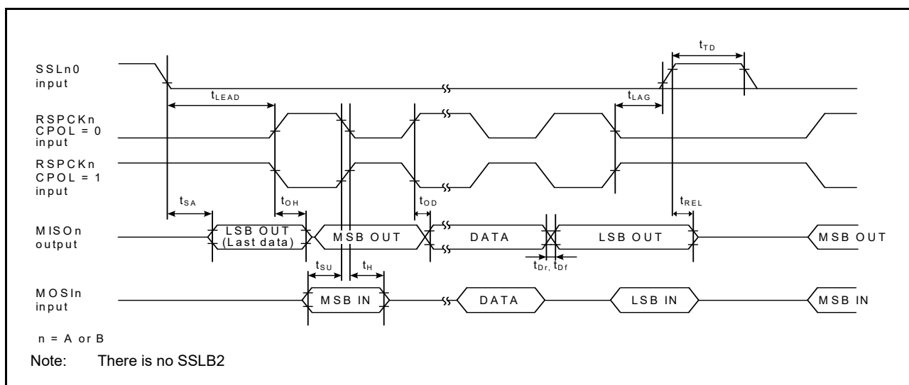
Figure 48.56 SPI timing (slave, CPHA = 1)
