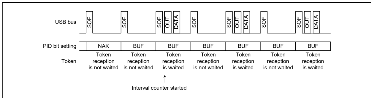
Figure 28.16 Relationship between frames and expected token reception when IITV \neq 0
