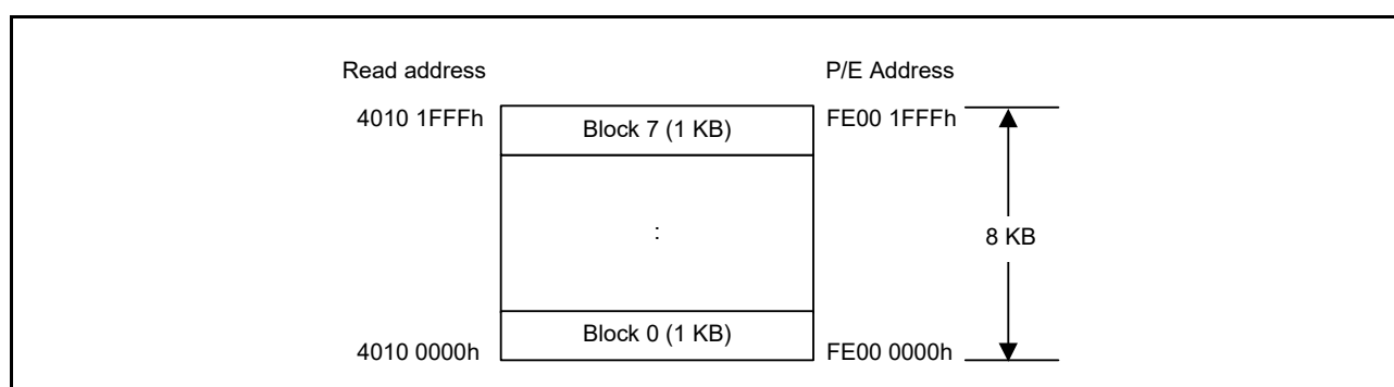
Figure 43.3 Mapping of the data flash memory
