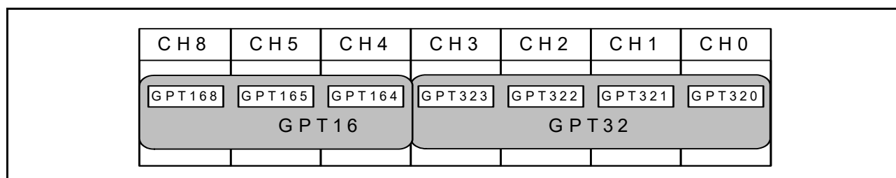
Figure 23.2 Association between GPT channels and module names
