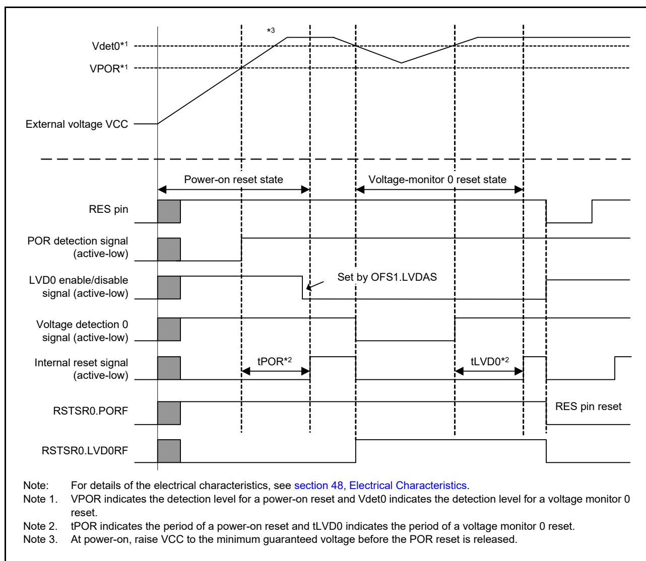
Figure 8.3 Example of voltage monitor 0 reset operation
