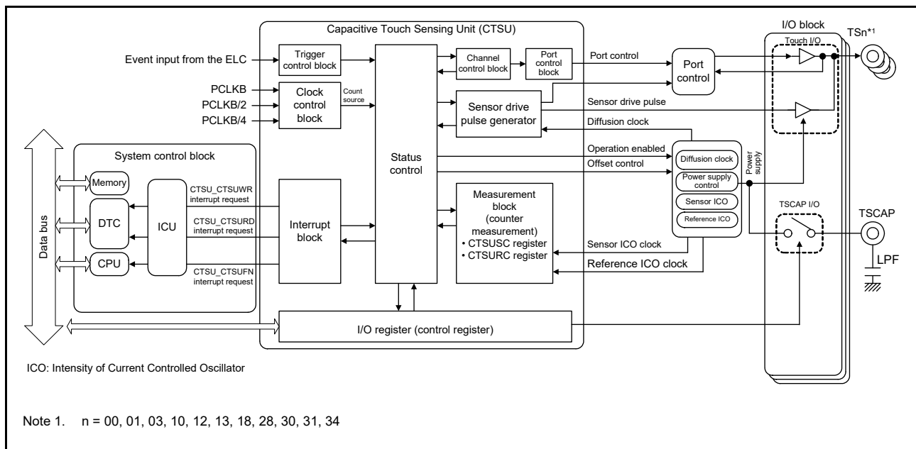
Figure 40.3 CTSUS block diagram
