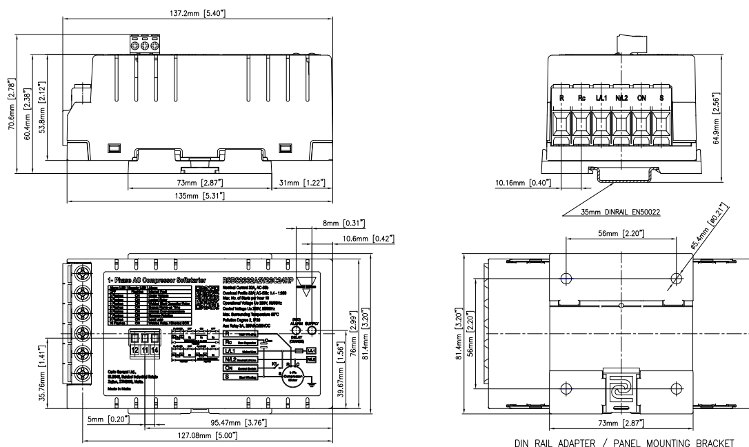
Fig. 4 RSBS2332A2V23C..HP
