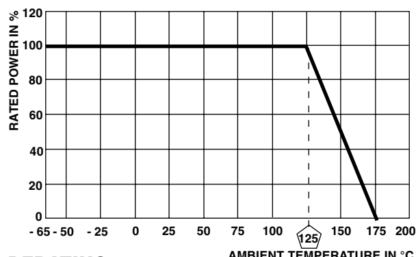
DERATING
