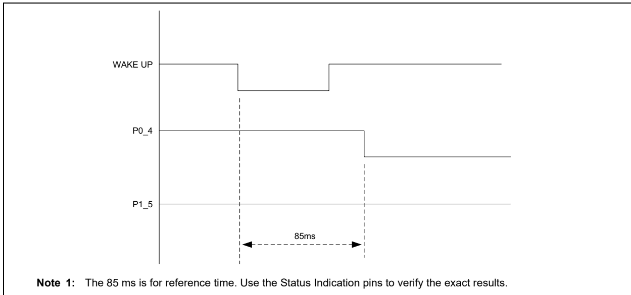
FIGURE 2-5: WAKE-UP TIME (1)
