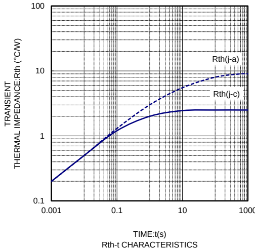
R_th-t CHARACTERISTICS
