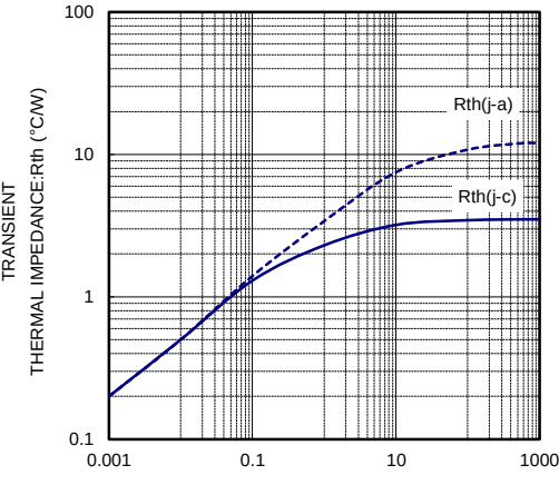
Rth-t CHARACTERISTICS
