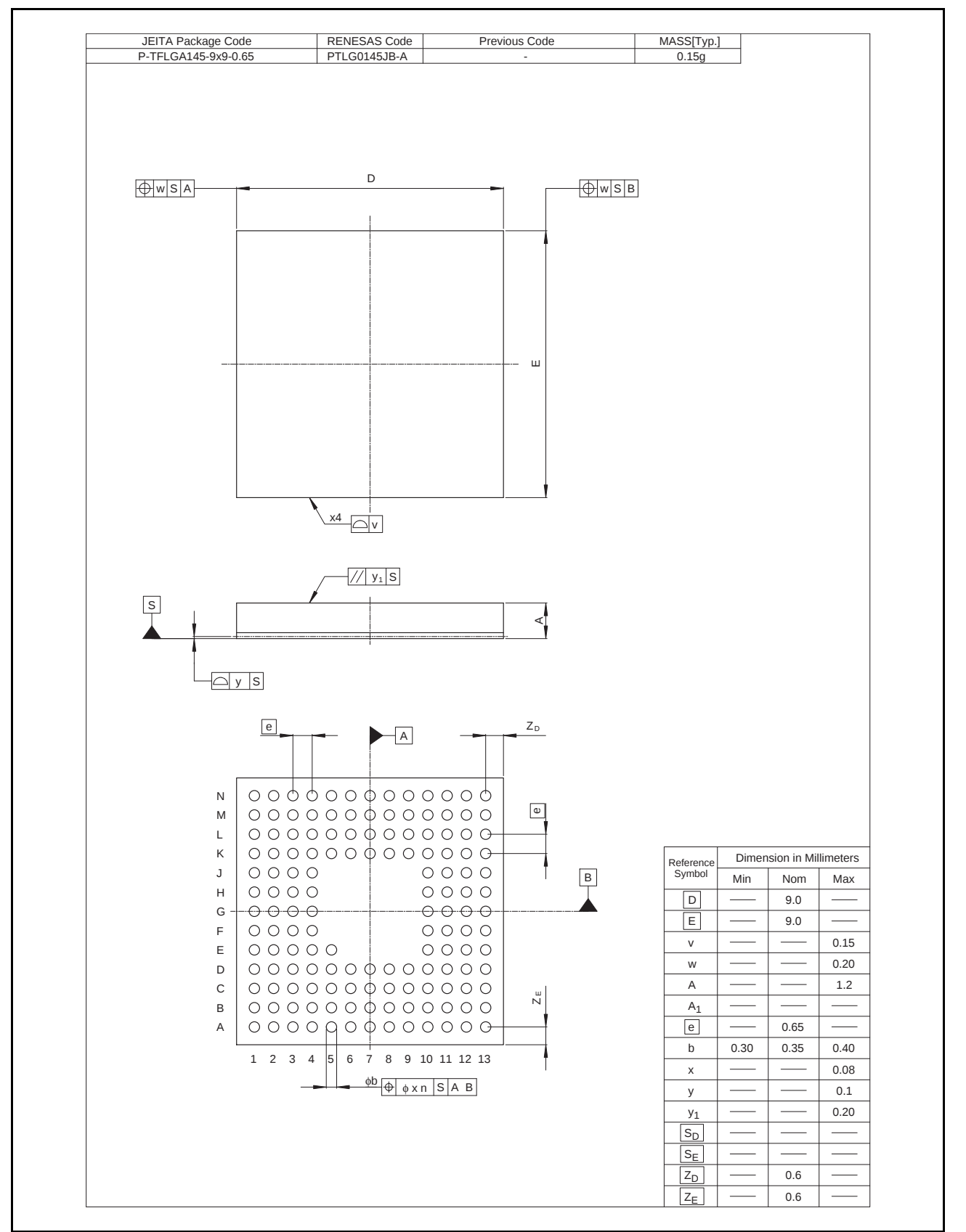
Figure B 145-Pin TFLGA (PTLG0145JB-A) Package Dimensions
