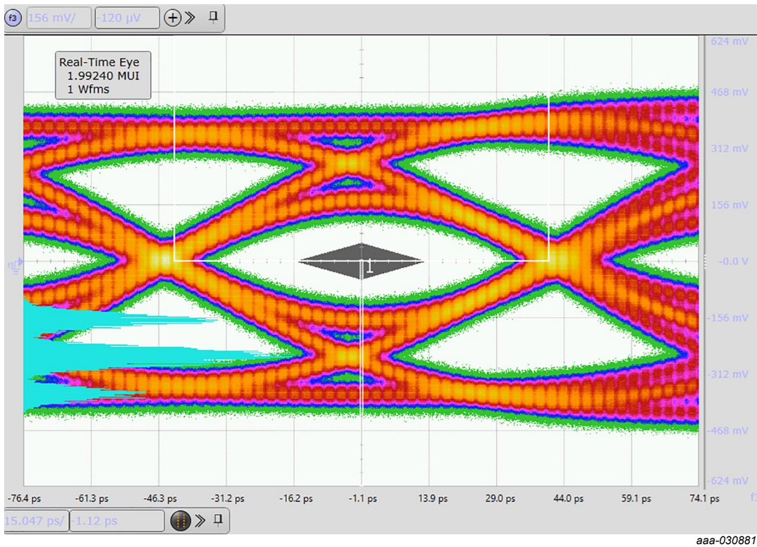
Fig. 10. HDMI 2.1 12G FRL TP2, Worst Case Model, 8 dB eye diagram, PCB with device; typical values
