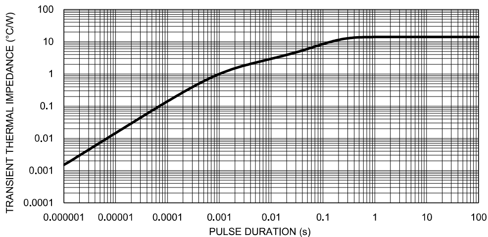
Fig.5 Typical Transient Thermal Impedance
