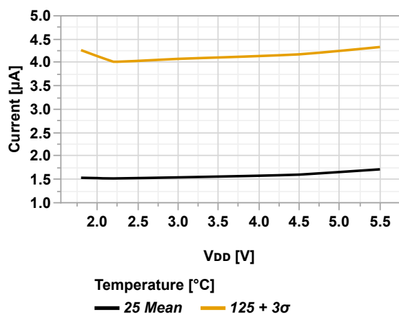
Figure 46-15. I_{PD} Base (VREGPM[1:0] = 'b01 = LP) vs. V_{DD}
