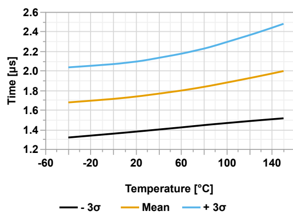
Figure 46-50. BOR Response Time vs. Temperature
