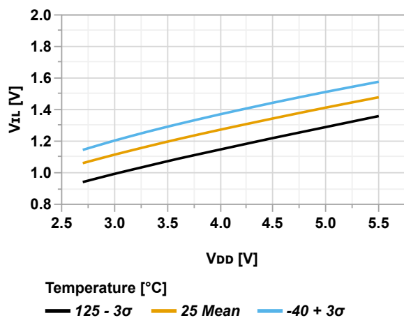
Figure 46-68. Input Pin with SMBus - Maximum V_{IL} vs. V_{DD} (SMBus 2.0)
