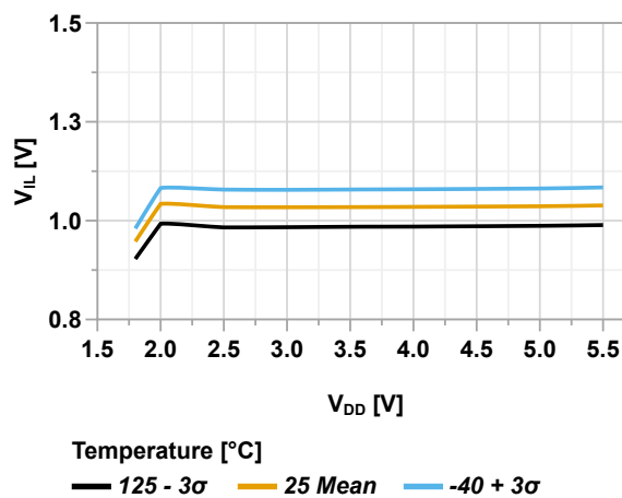
Figure 46-61. Input Pin with LVBUF - Maximum V_{IL} vs. V_{DD}
