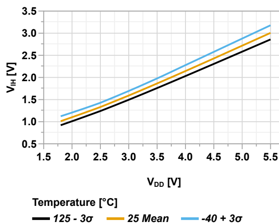
Figure 46-59. Input Pin with Schmitt Trigger - Minimum V_{IH} vs. V_{DD}
