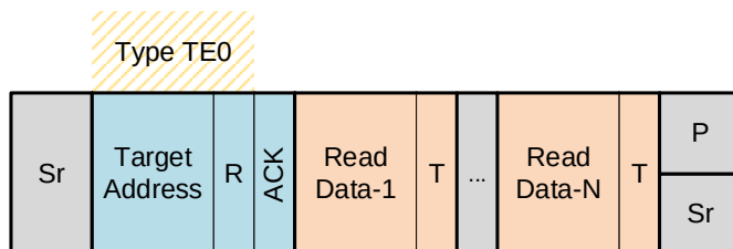
Figure 37-60. Private Read Transfer Initiated with Restart Condition (w/ 7'h7E) Error Type Frame Format
