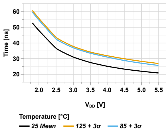
Figure 46-56. Rise Time (SLRxn = b ' 1) vs. V_{DD}
