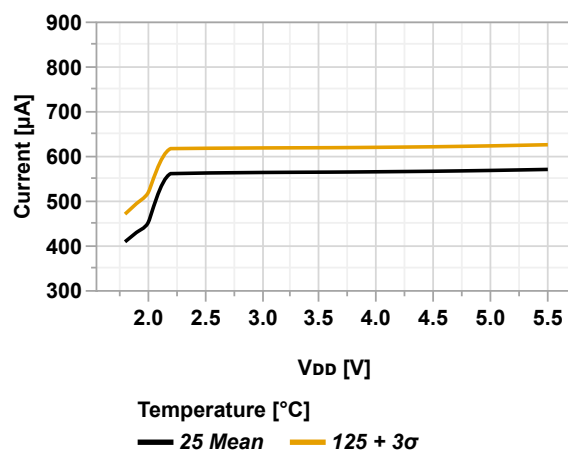
Figure 46-4. Active Power Consumption vs. V_{DD} (RSTOSC[2:0] = 'b110, OSCFRQ = 16 MHz, PMDx = 0xFF)
