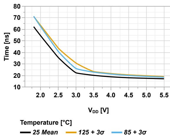
Figure 46-57. Rise Time (SLRxn = b ' 0) vs. V_{DD}
