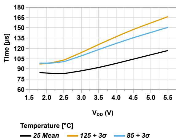
Figure 46-31. Wake-up Time (COSC[2:0] = 'b110, OSCFRQ = 4 MHz, VREGPM[1:0] = 'b01 = LP) vs. V_{DD}
