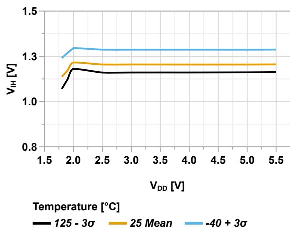
Figure 46-64. Input Pin with I 2 C Trigger - Maximum V_{IH} vs. V_{DD}
