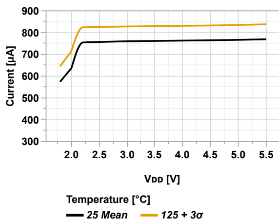
Figure 46-3. Active Power Consumption vs. V_{DD} (RSTOSC[2:0] = 'b110, OSCFRQ = 16 MHz, PMDx = 0x00)
