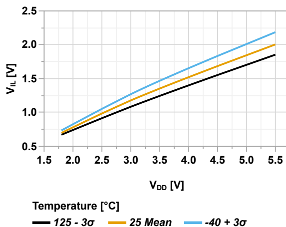
Figure 46-69. Reset Pin V_{IL} vs. V_{DD}
