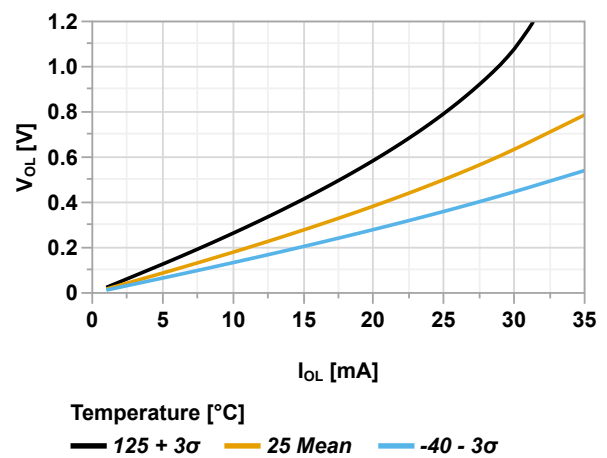
Figure 46-73. Output Pin - Maximum V_{OL} vs. Current, V_{DD} = 3.0V
