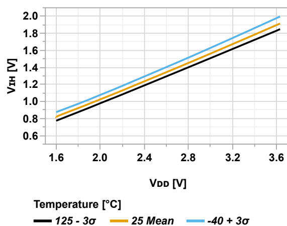
Figure 46-77. Input Pin with I3C Fast Schmitt Trigger - Maximum V_{IH} vs. V_{DD}
