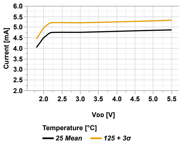
Figure 46-7. Active Power Consumption vs. V_{DD} (RSTOSC[2:0] = 'b010, EXTOSC[2:0] = 'b010, HS+PLL = 64 MHz, PMDx = 0x00)
