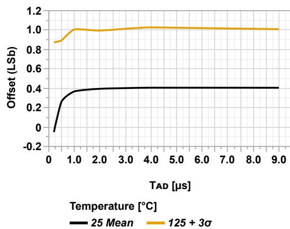
Figure 46-87. Offset Error vs. T_{AD} ( V_{REF+} = 3.0V = V_{DD} = 3.0V , CPON = 1)
