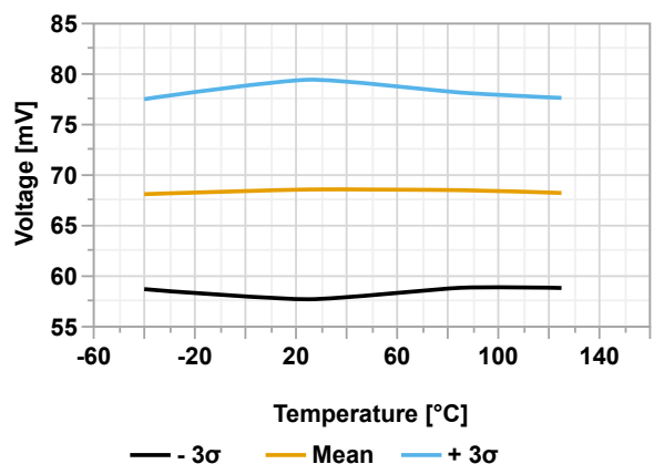
Figure 46-46. BOR Hysteresis (BORV[1:0] = 0) vs. Temperature
