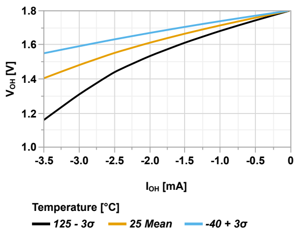
Figure 46-72. Output Pin - Minimum V_{OH} vs. Current, V_{DD} = 1.8V
