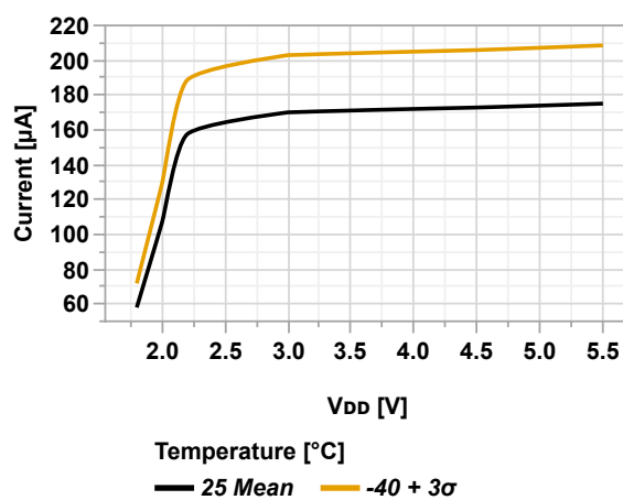
Figure 46-16. I_{PD} Base (VREGPM[1:0] = 'b00 = HP) vs. V_{DD}
