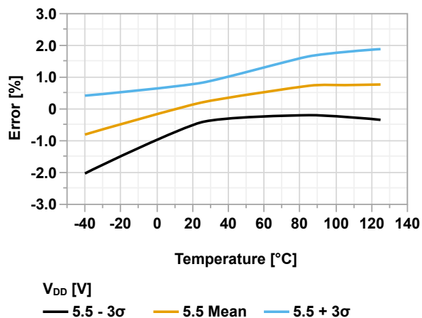
Figure 46-83. ADFVR Voltage Error vs. Temperature ( V_{DD} = 5.5V , V_{REF} = 4.096V )
