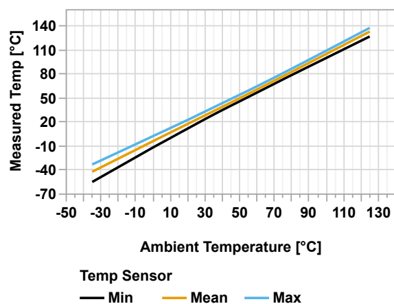
Figure 46-96. Temperature Sensor Characteristics, V_{DD} = 3.0V
