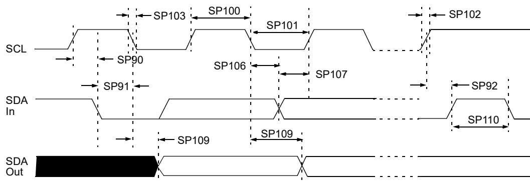
Figure 45-18. I 2 C Bus Data Timing
