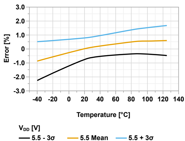
Figure 46-83. ADFVR Voltage Error vs. Temperature ( V_{DD} = 5.5V , V_{REF} = 4.096V )
