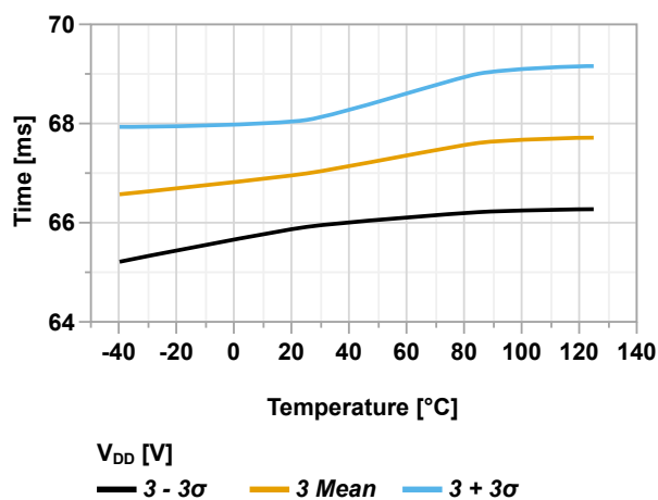
Figure 46-38. Start-up Time vs. Temperature (PWRTS[1:0] = 0x2, V_{DD} = 3.0V)
