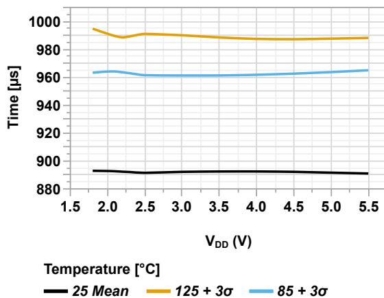
Figure 46-27. Wake-up Time (COSC[2:0] = 'b101, FOSC = 31 kHz, VREGPM[1:0] = 'b11 = ULP + Extended Temperature Range) vs. V_{DD}
