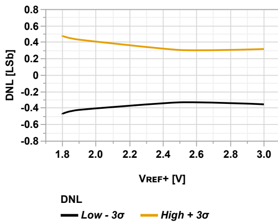
Figure 46-90. DNL vs. V_{REF+} ( T_{AD} = 1 \mu s , V_{DD} = 3.0V , T = 125^\circ C , CPON = 1)
