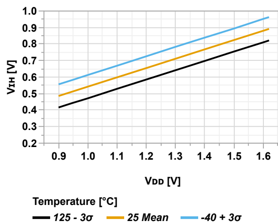
Figure 46-79. Input Pin with I3C LV Trigger - Maximum V_{IH} vs. V_{DD}
