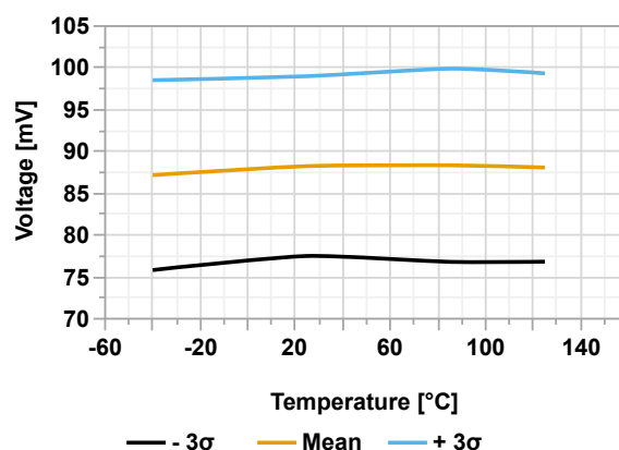
Figure 46-49. BOR Hysteresis (BORV[1:0] = 3) vs. Temperature
