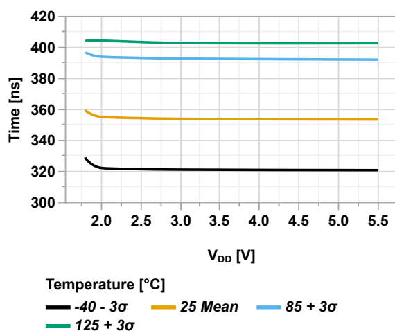
Figure 46-35. Minimum Reset Pulse Width vs. V_{DD}
