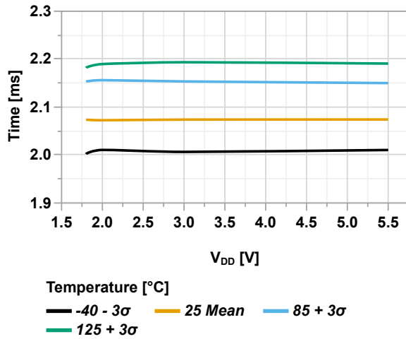
Figure 46-51. WWDT Time-Out Period over V_{DD} and Temperature (PS[4:0] = 0x01)
