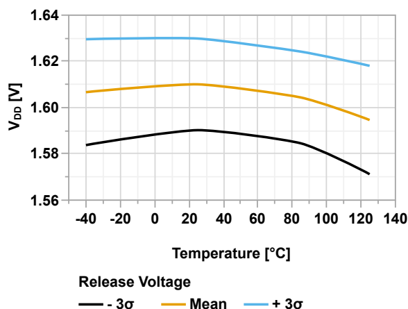
Figure 46-40. POR Release Voltage vs. Temperature
