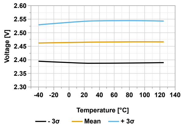
Figure 46-43. BOR Threshold Level (BORV[1:0] = 1) vs. Temperature
