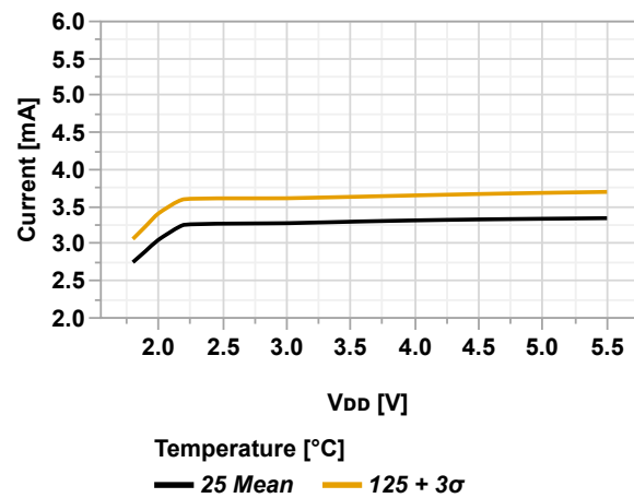
Figure 46-8. Active Power Consumption vs. V_{DD} (RSTOSC[2:0] = 'b010, EXTOSC[2:0] = 'b010, HS+PLL = 64 MHz, PMDx = 0xFF)
