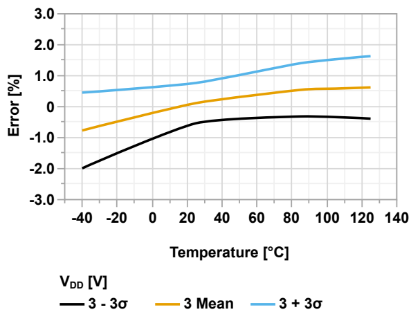
Figure 46-85. ADFVR Voltage Error vs. Temperature ( V_{DD} = 3.0V , V_{REF} = 2.048V )
