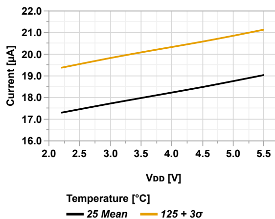
Figure 46-24. I_{PD} HLVD vs. V_{DD}
