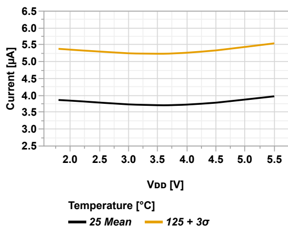
Figure 46-19. I_{PD} SOSC (SOSCPWR = High Power) vs. V_{DD}
