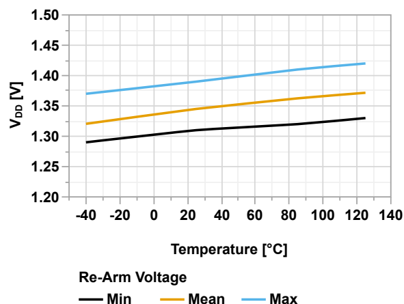
Figure 46-41. POR Re-Arm Voltage vs. Temperature
