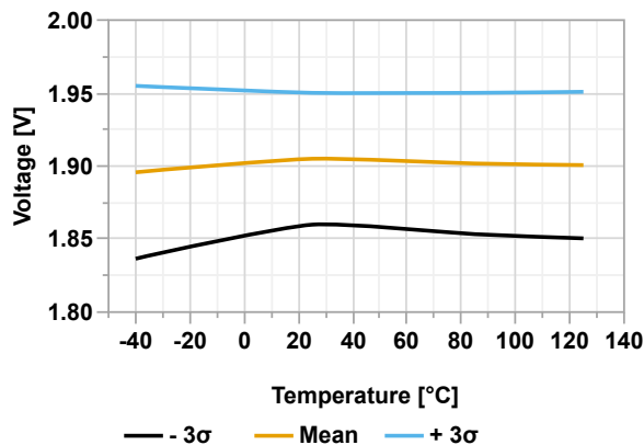
Figure 46-42. BOR Threshold Level (BORV[1:0] = 0) vs. Temperature
