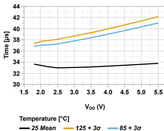
Figure 46-32. Wake-up Time (COSC[2:0] = 'b110, OSCFRQ = 16 MHz, VREGPM[1:0] = 'b01 = LP) vs. V_{DD}
