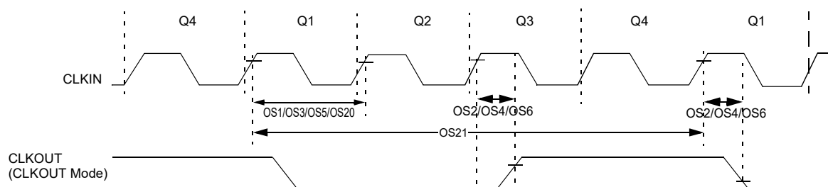
Figure 45-4. Clock Timing
