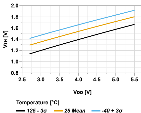
Figure 46-67. Input Pin with SMBus - Maximum V_{IH} vs. V_{DD} (SMBus 2.0)
