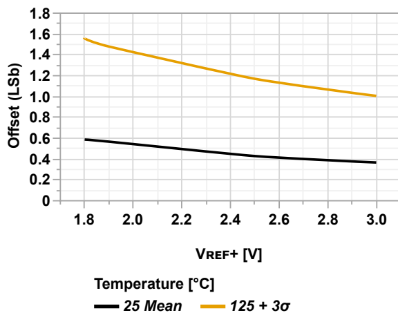
Figure 46-86. Offset Error vs. V_{REF+} ( T_{AD} = 1 \mu s , V_{DD} = 3.0V , CPON = 1)
