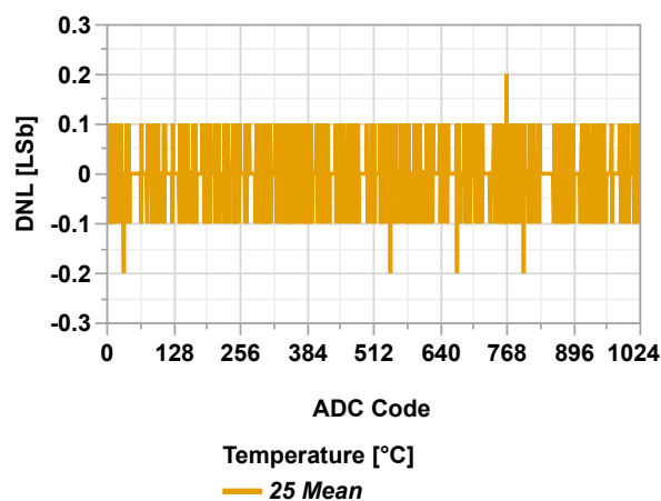
Figure 46-95. DNL vs. ADC Code ( T_{AD} = 1 \mu s , V_{DD} = 3.0V )
