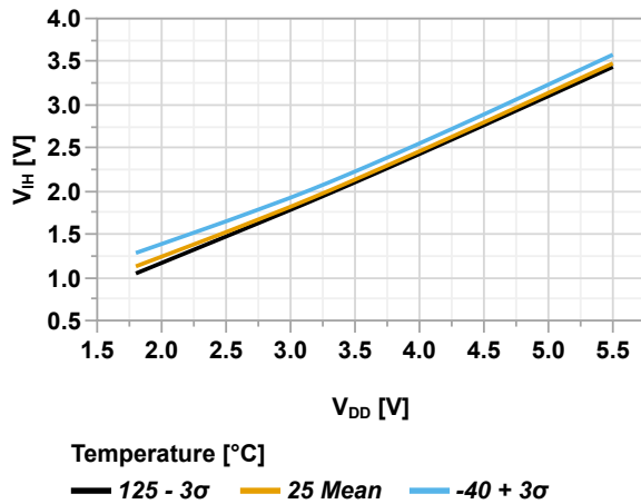
Figure 46-70. Reset Pin V_{IH} vs. V_{DD}
