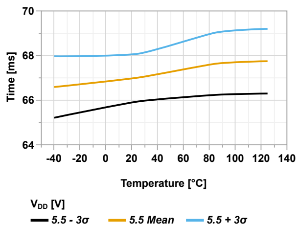
Figure 46-39. Start-up Time vs. Temperature (PWRTS[1:0] = 0x2, V_{DD} = 5.5V)
