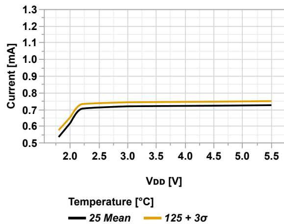
Figure 46-12. Doze Power Consumption vs. V_{DD} (RSTOSC[2:0] = 'b110, OSCFRQ = 16 MHz, PMDx = 0xFF)
