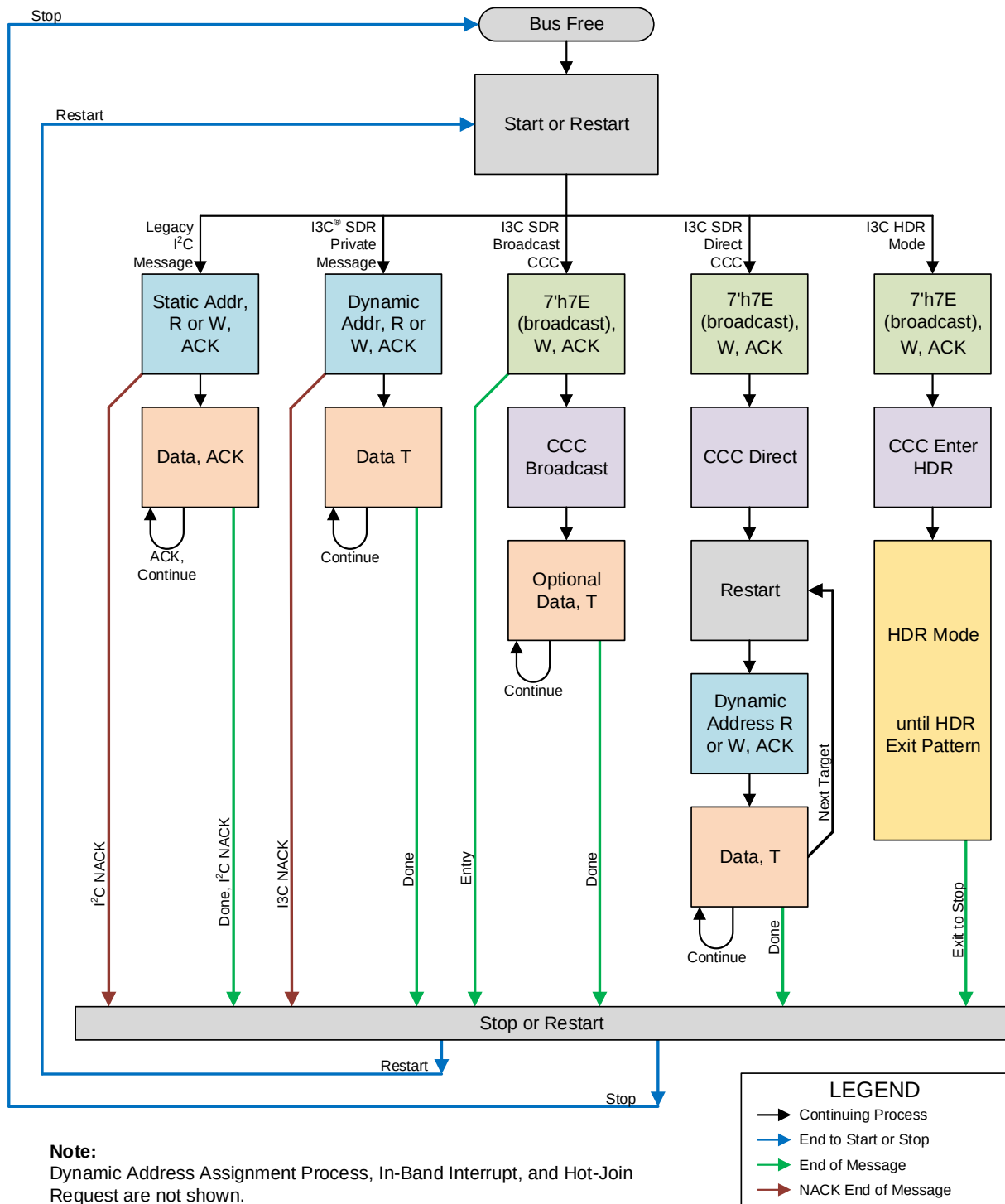
Figure 37-7. I3C® Target Bus Communication Flowchart
