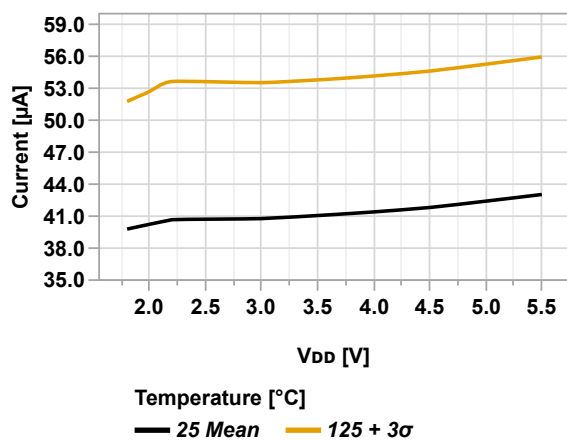
Figure 46-15. I_{PD} Base (VREGPM[1:0] = 'b01 = LP) vs. V_{DD}
