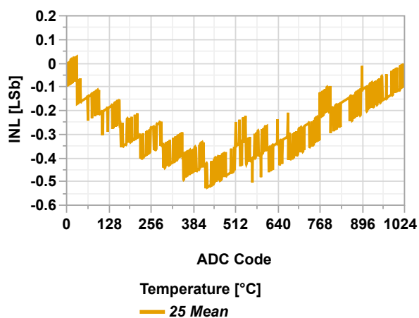
Figure 46-94. INL vs. ADC Code ( T_{AD} = 1 \mu s , V_{DD} = 3.0V )
