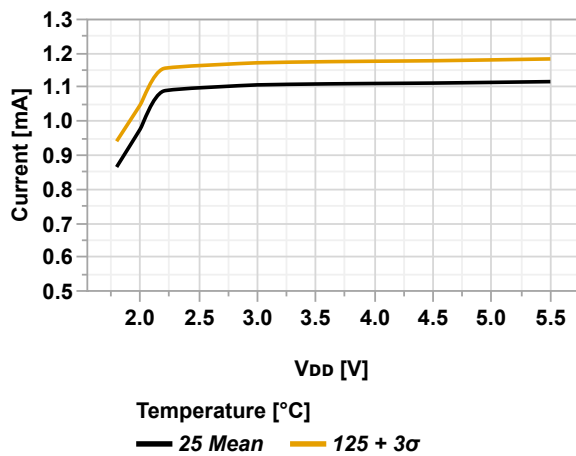
Figure 46-11. Doze Power Consumption vs. V_{DD} (RSTOSC[2:0] = 'b110, OSCFRQ = 16 MHz, PMDx = 0x00)
