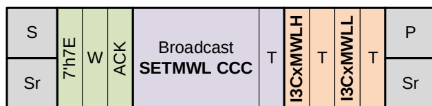
Figure 37-38. Broadcast Write SETMWL Frame Format
