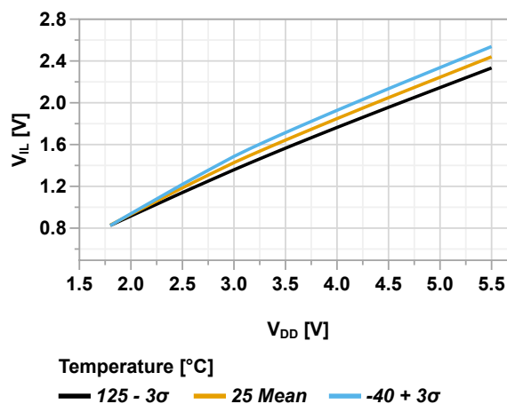
Figure 46-65. Input Pin with SMBus - Maximum V_{IL} vs. V_{DD} (SMBus 3.0)
