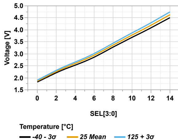
Figure 46-53. HLVD Positive Edge SEL[3:0] vs. Temperature
