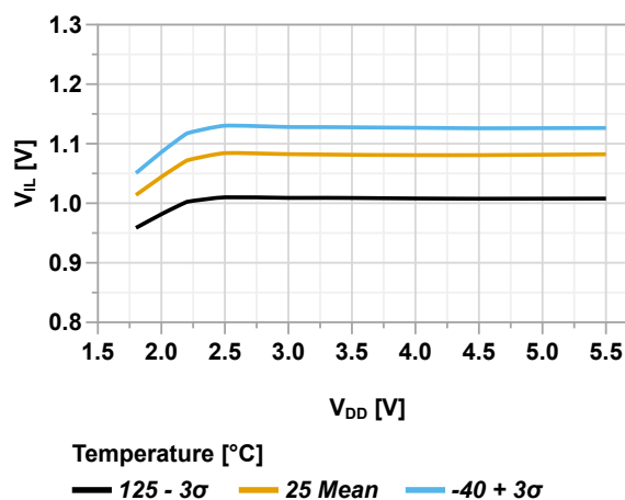
Figure 46-65. Input Pin with SMBus - Maximum V_{IL} vs. V_{DD} (SMBus 3.0)
