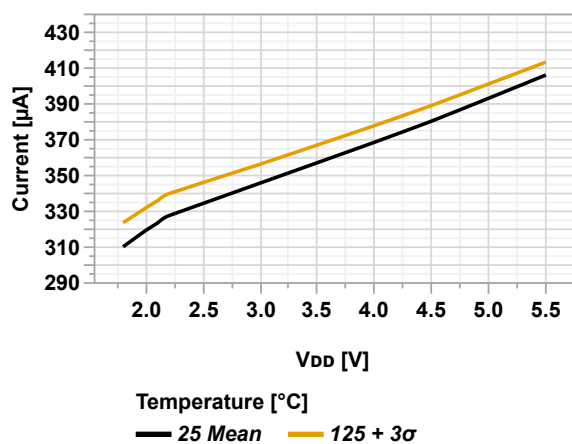
Figure 46-23. I_{PD} ADC vs. V_{DD}
