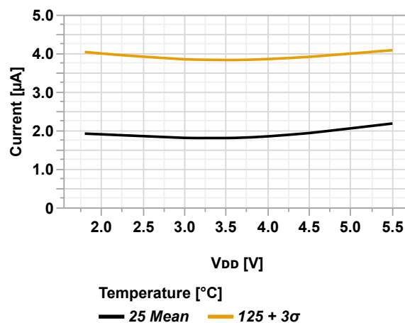
Figure 46-20. I_{PD} LPBOR vs. V_{DD}
