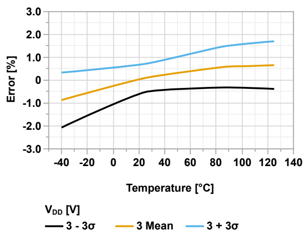
Figure 46-84. ADFVR Voltage Error vs. Temperature ( V_{DD} = 3.0V , V_{REF} = 1.024V )
