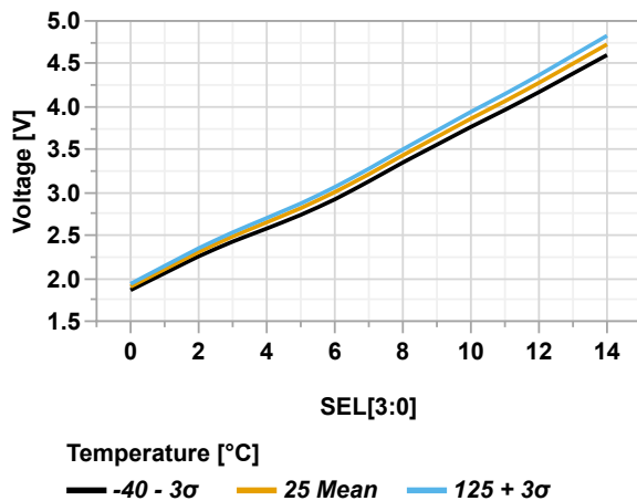
Figure 46-52. HLVD Negative Edge SEL[3:0] vs. Temperature
