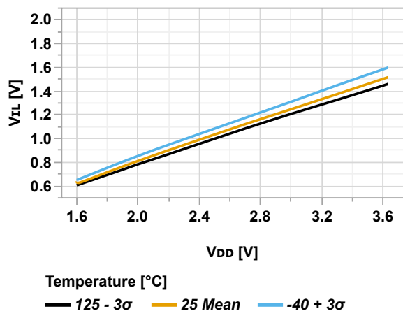
Figure 46-80. Input Pin with I3C LV Trigger - Maximum V_{IL} vs. V_{DD}
