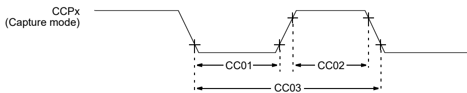
Figure 45-12. Capture/Compare/PWM Timings (CCP)
