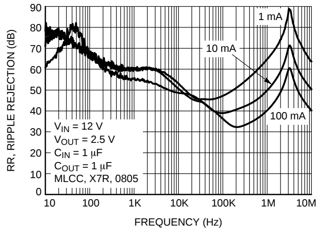
Figure 12. Power Supply Rejection Ratio vs. Current, V_{IN} = 12\text{ V} , C_{OUT} = 1\text{ }\mu\text{F}
