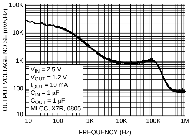
Figure 13. Output Voltage Noise Spectral Density for V_{OUT} = 1.2\text{ V} , I_{OUT} = 10\text{ mA} , C_{OUT} = 1\text{ }\mu\text{F}
