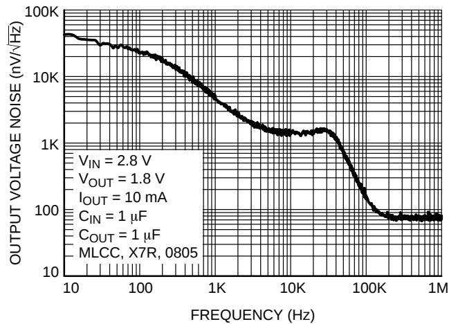
Figure 14. Output Voltage Noise Spectral Density for V_{OUT} = 1.8\text{ V} , I_{OUT} = 10\text{ mA} , C_{OUT} = 1\text{ }\mu\text{F}
