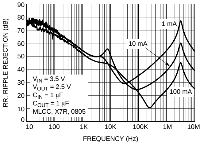
Figure 11. Power Supply Rejection Ratio vs. Current, V_{IN} = 3.5\text{ V} , C_{OUT} = 1\text{ }\mu\text{F}
