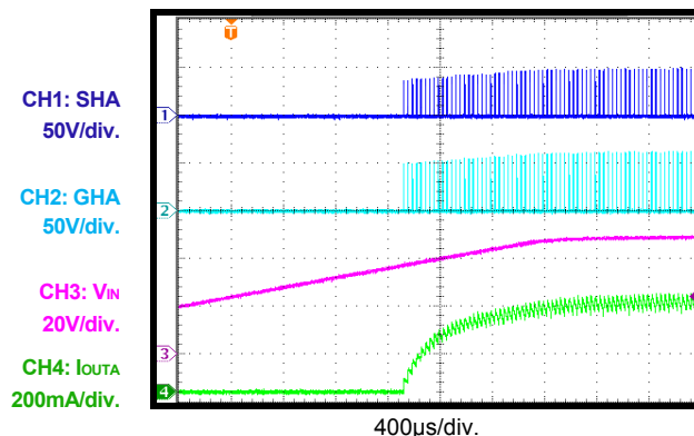
Power Ramp-Up
