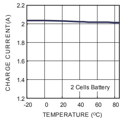
Charge Current vs. Temperature
