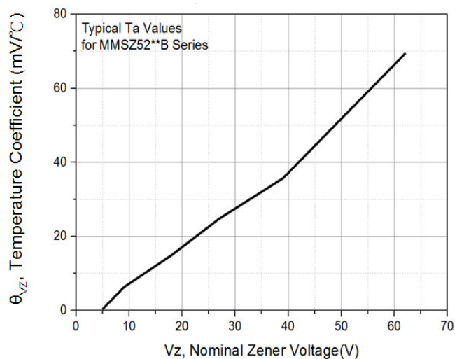
Fig. 6 Temperature Coefficients Curve.
