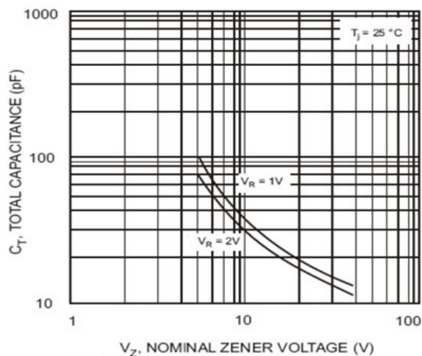
Fig. 2 Total Capacitance vs Nominal Zener Voltage
