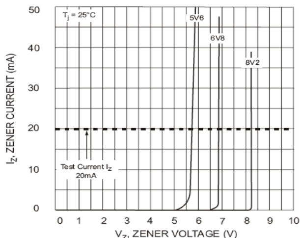
Fig. 4 Zener Breakdown Characteristics
