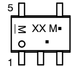
SC-88A / SOT-353 / SC-70 DF SUFFIX CASE 419A-02
