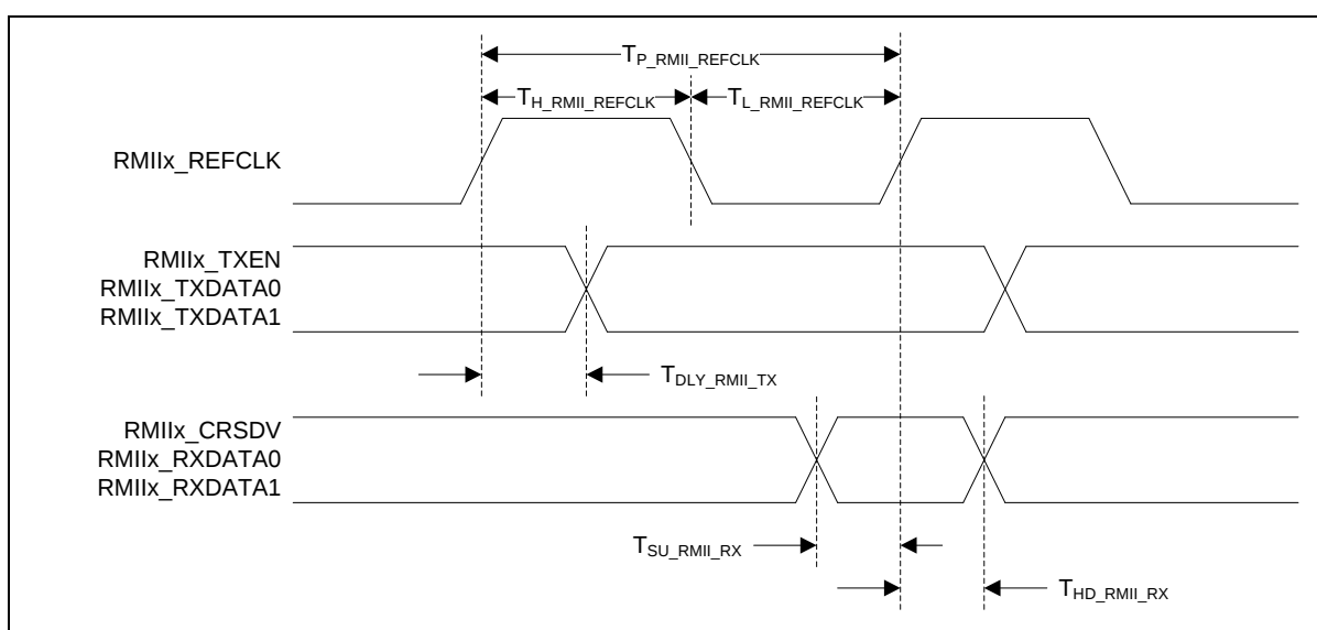
Figure 8.13-1 RMII Interface Timing Diagram
