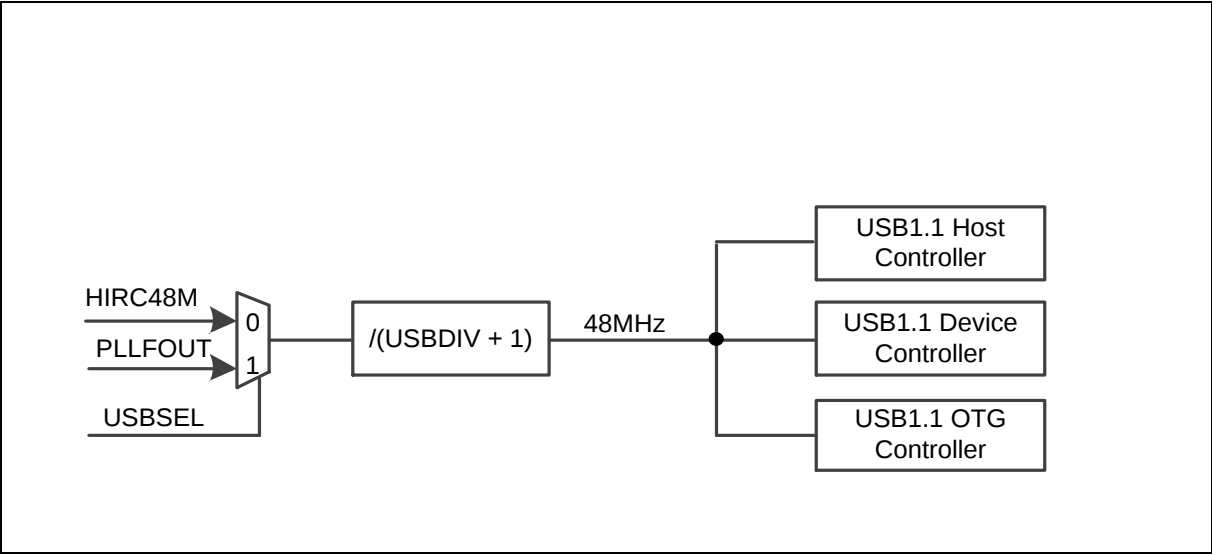
Figure 6.3-9 USB Clock Source (M48xGC/M48xE8)
