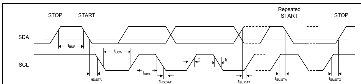
Figure 8.7-1 I 2 C Timing Diagram
