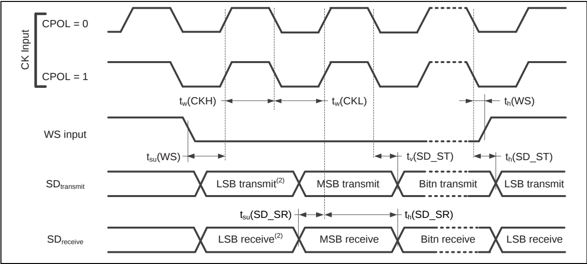
Figure 8.9-2 I²S Slave Mode Timing Diagram
