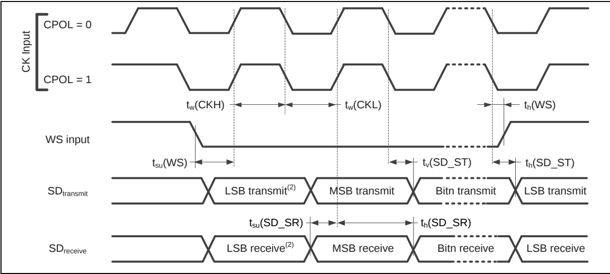
Figure 9.6-4 I²S Slave Mode Timing Diagram
