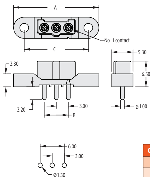
Recommended PC Board Pattern
