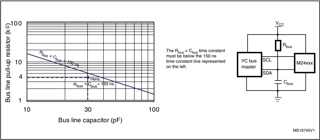
Figure 11. Maximum R_{bus} value versus bus parasitic capacitance C_{bus} ) for an I 2 C bus at maximum frequency f_C = 1\text{ MHz}
