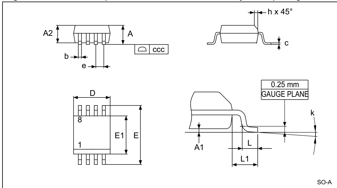
Figure 14. SO8N – 8 lead plastic small outline, 150 mils body width, package outline
