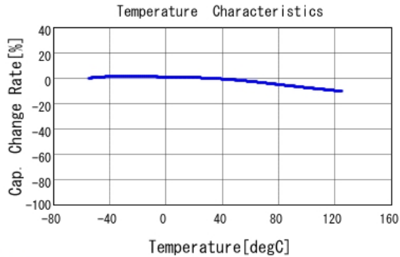
■ KRM55WR71J226MH01 C-Temp. capchange, DCOV, ACO, 5Vrms
