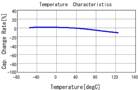
■ KRM55WR71H336MH01 C-Temp. capchange, DCOV, ACO, 5Vrms
