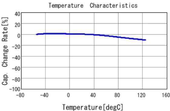
■ KRM55TR71H226MH01 C-Temp. capchange, DC0V, AC0.5Vrms
