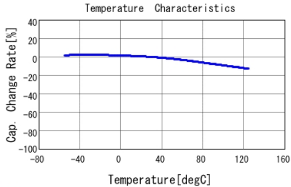
■ KRM55TR71E336MH01 C-Temp. capchange, DC0V, AC0.5Vrms
