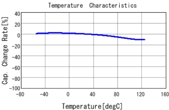
■ KRM55QR71E336KH01 C-Temp. capchange, DC0V, AC0.5Vrms
