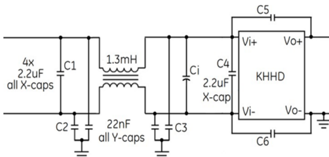
Figure 17. Suggested Configuration for EN55032 Class B.
