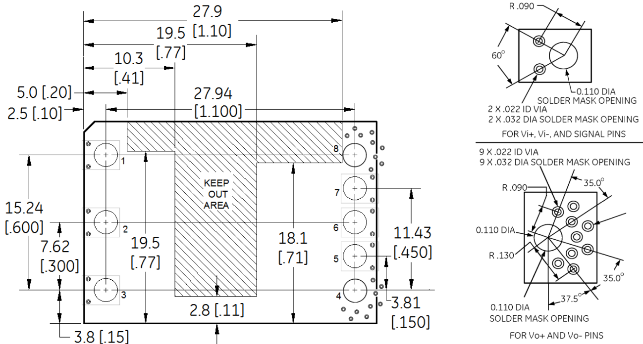
Surface Mount Pad Layout
