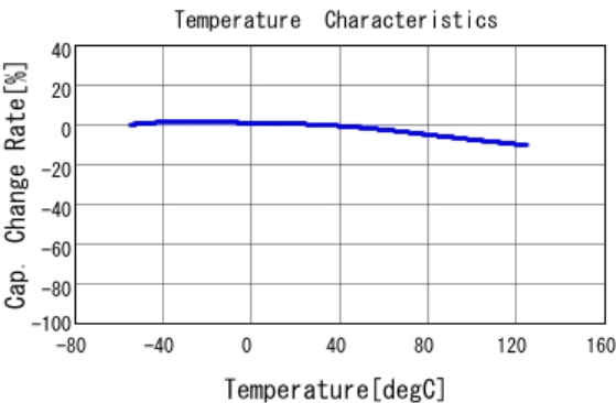
■ KCM55WR72A226MH01 C-Temp. capchange, DC0V, AC0.5Vrms
