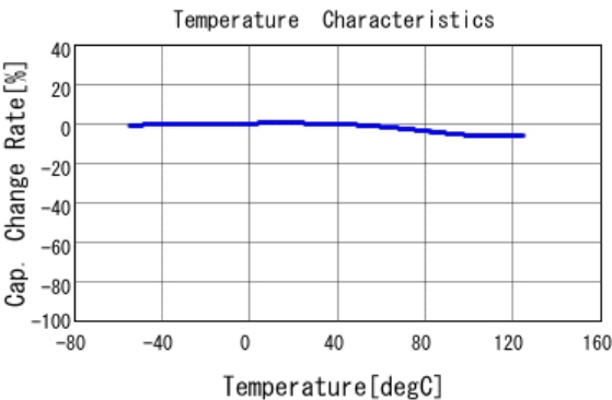
■ KCM55WR72A156MH01 C-Temp. capchange, DC0V, AC0.5Vrms
