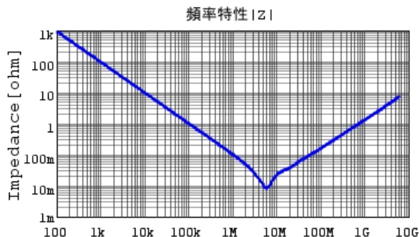
GRT155R61E225KE13 |Z| DCOV, 25degC
