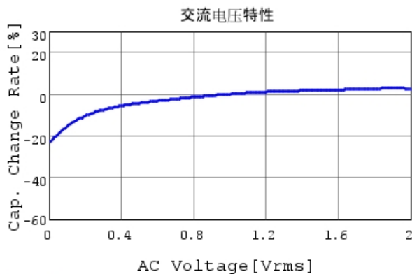
GRT155R61E225KE13 C-AC Voltage capchange, DC
