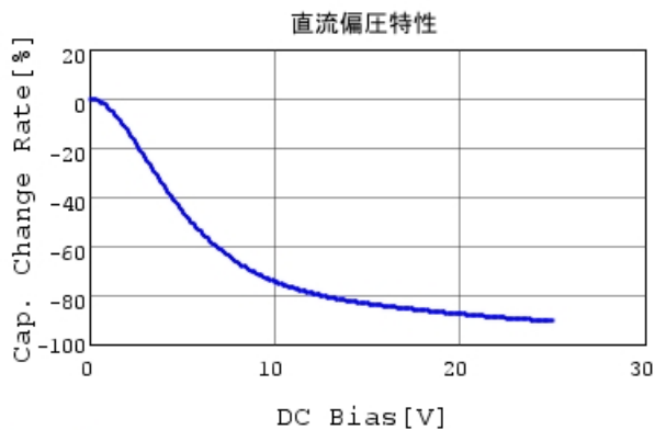
GRT155R61E225KE13 C-DC bias capchange, 25.00
