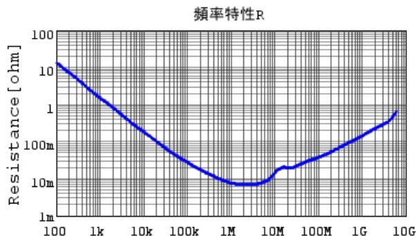
GRT155R61E225KE13 R DCOV, 25degC
