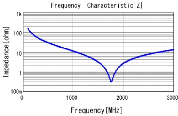
■ GRM31A7U2J100JW31 |Z| DCOV, 25degC
