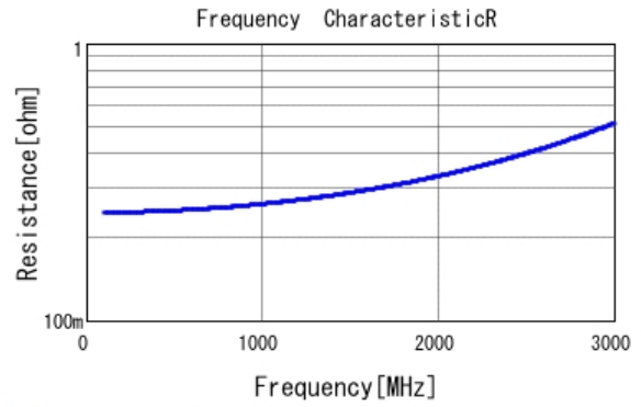
■ GRM31A7U2J100JW31 R DCOV, 25degC
