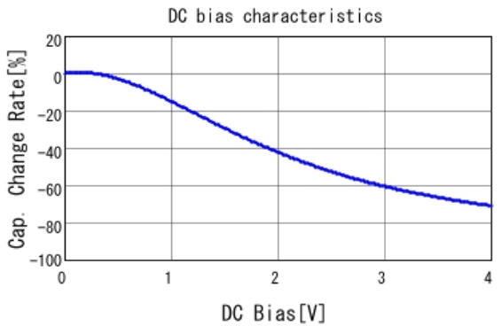
■ GRM188R60G226MEA0 C-DC bias capchange, 25.0degC, AC0.
