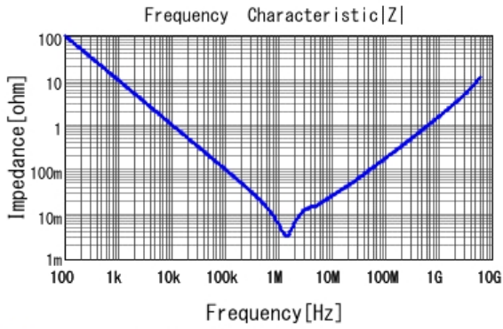
■ GRM188R60G226MEA0 |Z| DCOV, 25degC
