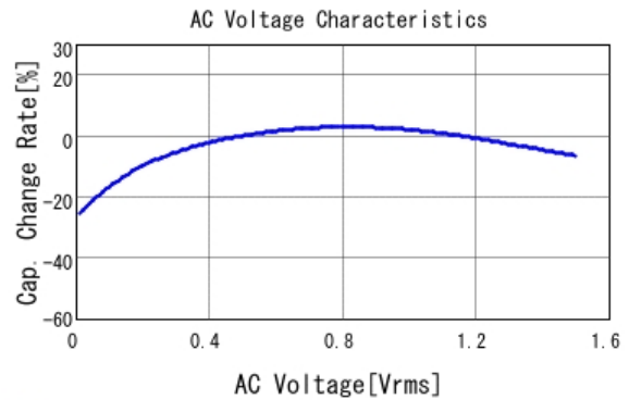
■ GRM188R60G226MEA0 C-AC Voltage capchange, DCOV, 25.0d
