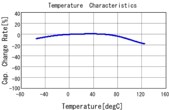
■ GRM188C70J225KE20 C-Temp. capchange, DCO. 0V, ACO. 5V rm
