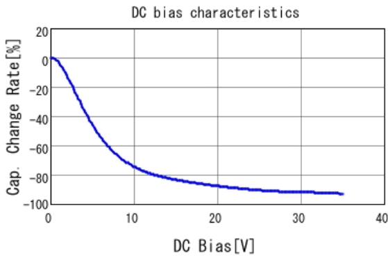
■ GRM155R6YA225ME11 C-DC bias capchange, 25.0degC, AC1V
