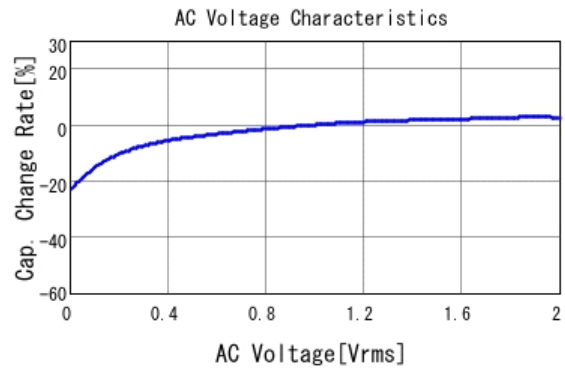
■ GRM155R6YA225ME11 C-AC Voltage capchange, DCOV, 25.0d
