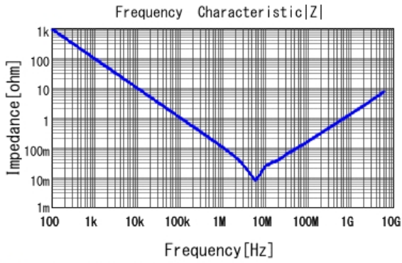
■ GRM155R6YA225ME11 |Z| DCOV, 25degC
