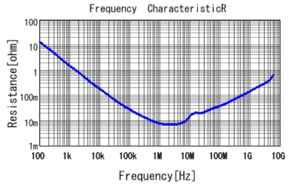
■ GRM155R6YA225ME11 R DCOV, 25degC
