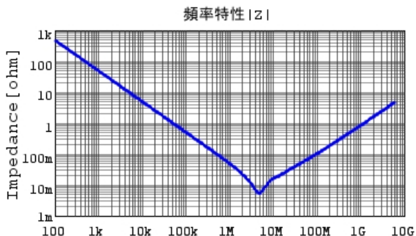
GRM035R60G475ME15 |Z| DCOV, 25degC
