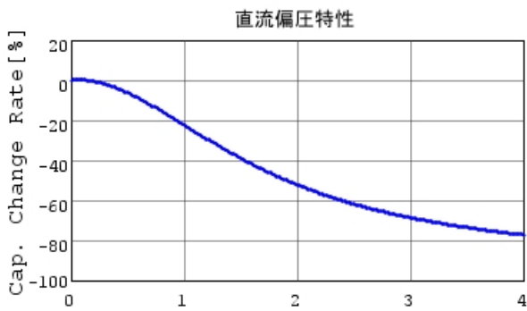
GRM035R60G475ME15 C-DC bias capchange, 25.0C
