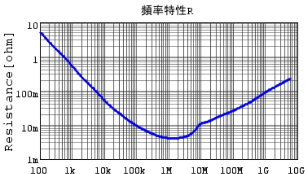
GRM035R60G475ME15 R DCOV, 25degC
