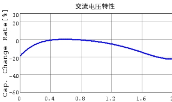
GRM035R60G475ME15 C-AC Voltage capchange, DC
