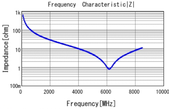
■ GRM0335C2A2R5WA01 |Z| DCOV, 25degC
