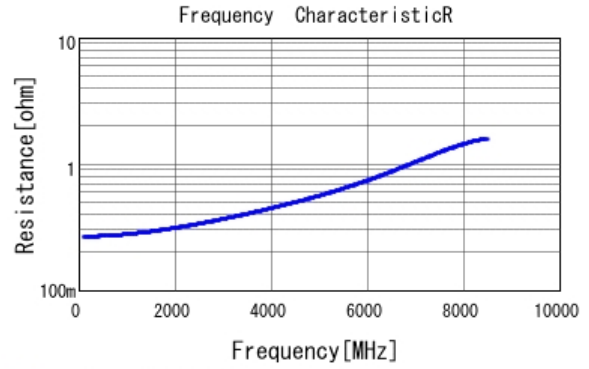
■ GRM0335C2A2R5WA01 R DCOV, 25degC
