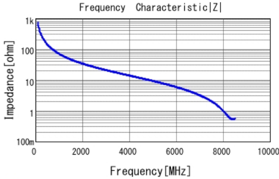
■ GRM0225C1H2R2CA03 |Z| DCOV, 25degC
