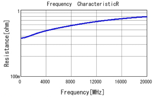
■ GRM0225C1H1R4BA03 R DC0V, 25degC
