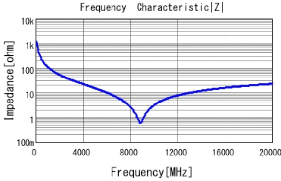
■ GRM0225C1H1R4BA03 |Z| DC0V, 25degC
