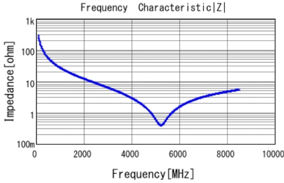
■ GRM0225C1E5R6DA03 |Z| DC0V, 25degC
