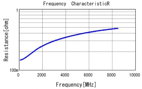
■ GRM0225C1E5R6DA03 R DC0V, 25degC
