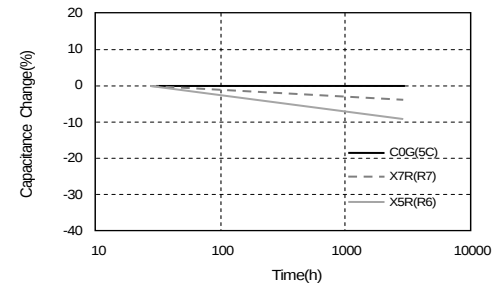
[ Example of Change Over Time (Aging characteristics) ]
