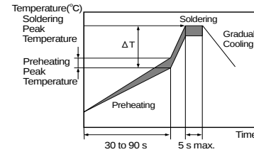
[Allowable Flow Soldering Temperature and Time]
