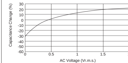
[Example of AC Voltage Characteristics]
