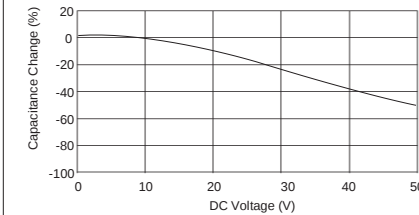
[Example of DC Voltage Characteristics]
