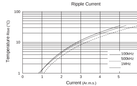
[Example of Temperature Rise (Heat Generation) in Chip Multilayer Ceramic Capacitors in Contrast to Ripple Current] Sample: R(R1) characteristics 10 \mu F, Rated voltage: DC10V
