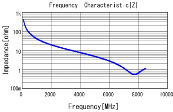
■ GRM0115C1C3R9CE01 |Z| DC0V, 25degC
