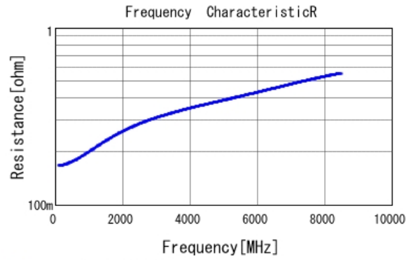
■ GRM0115C1C3R9CE01 R DC0V, 25degC
