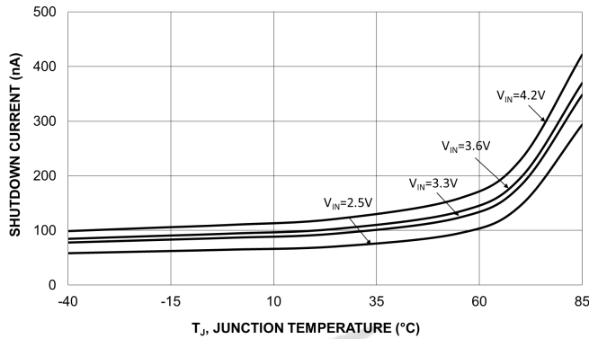
Figure 9. Shutdown Current vs. Temperature GLF73910-AD01, GLF73910-AD01C, GLF73910-BD01
