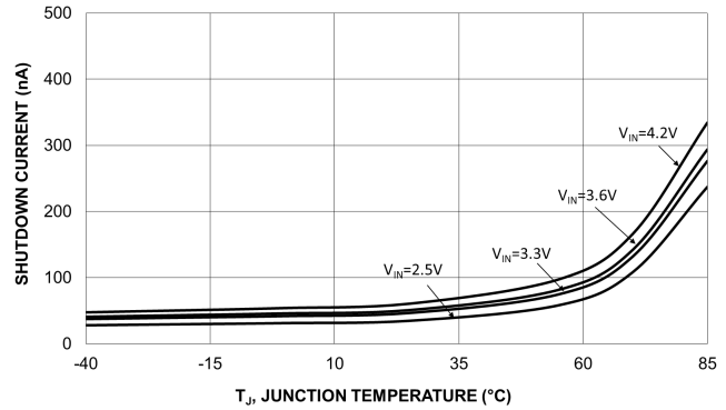
Figure 10. Shutdown Current vs. Temperature GLF73911-AD01
