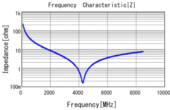
■ GJM0335C2A7R3BB01 |Z| DC0V, 25degC
