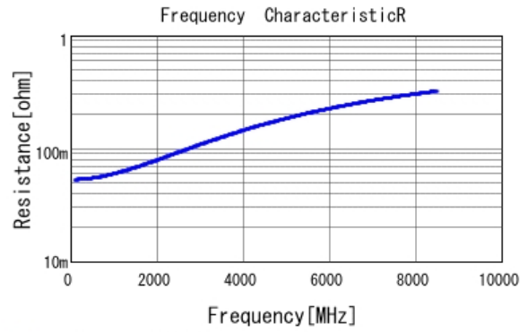
■ GJM0335C2A7R3BB01 R DC0V, 25degC
