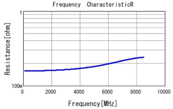
■ GJM0335C2A2R5CB01 R DC0V, 25degC
