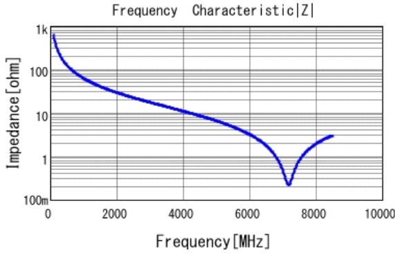
■ GJM0335C2A2R5CB01 |Z| DC0V, 25degC
