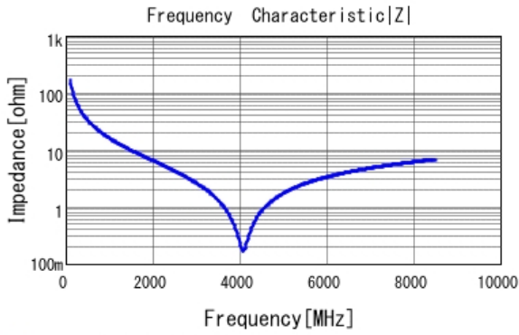
■ GJM0225C1C9R3DB01 |Z| DCOV, 25degC
