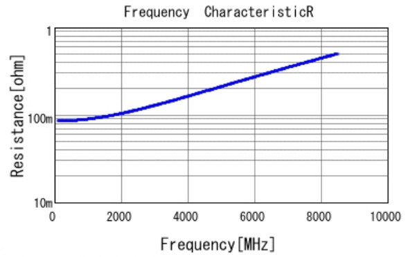
■ GJM0225C1C9R3DB01 R DCOV, 25degC
