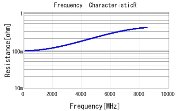
■ GJM0225C1C7R4DB01 R DC0V, 25degC
