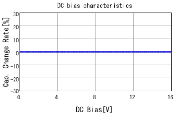
■ GJM0225C1C7R4DB01 C-DC bias capchange, 25.0degC, AC1V
