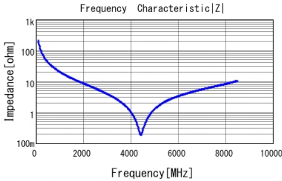
■ GJM0225C1C7R4DB01 |Z| DC0V, 25degC
