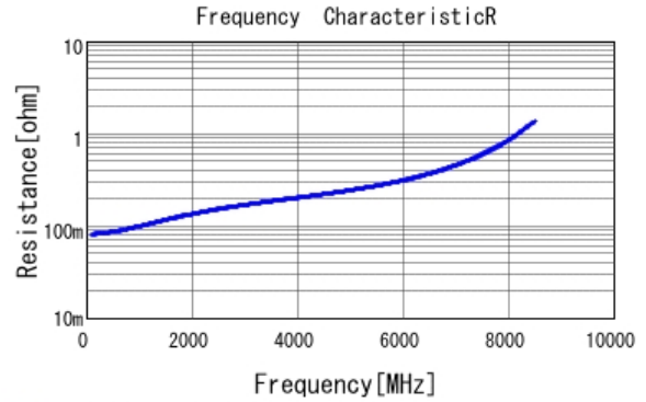
■ GCQ1555C1H6R9BB01 R DC0V, 25degC
