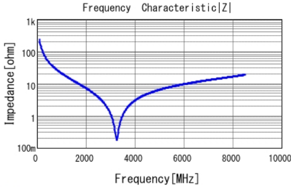
■ GCQ1555C1H6R9BB01 |Z| DC0V, 25degC
