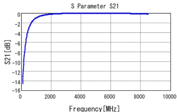
■ GCQ1555C1H3R0WB01 S21 DC0V, 25degC
