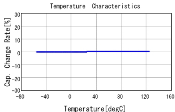
■ GCQ1555C1H3R0WB01 C-Temp. capchange, DC0V, AC1Vrms
