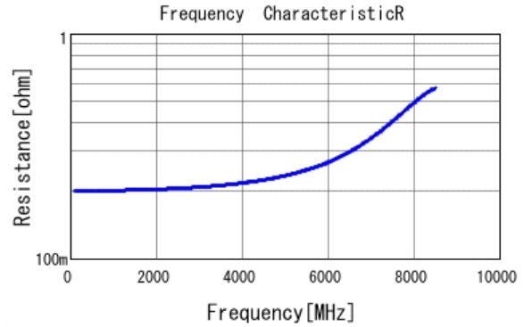
■ GCQ1555C1H1R9WB01 R DC0V, 25degC
