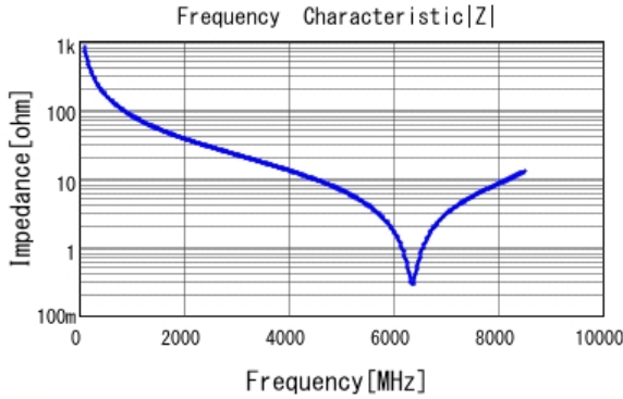
■ GCQ1555C1H1R9WB01 |Z| DC0V, 25degC
