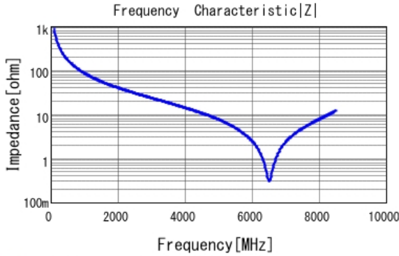
■ GCQ1555C1H1R8WB01 |Z| DCOV, 25degC
